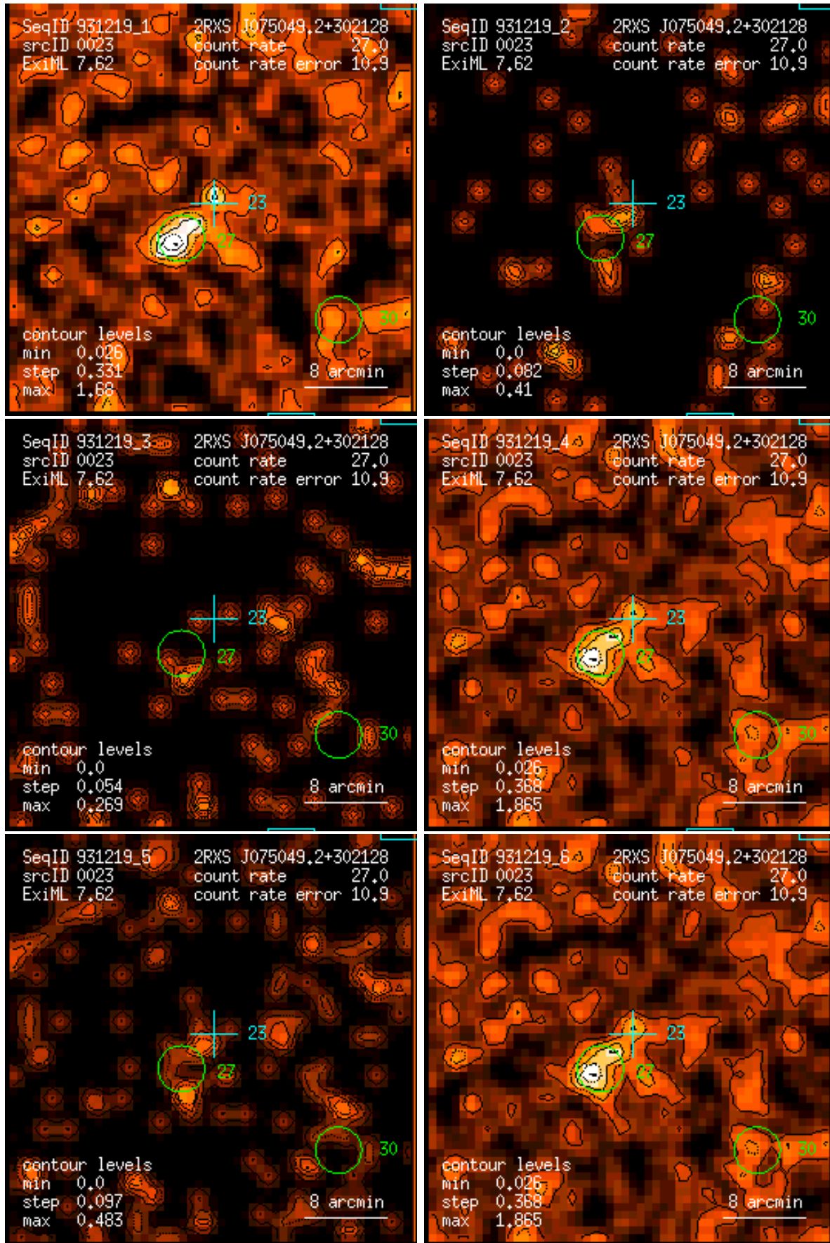
Figure 23: RASS 931219: detection 0023: band rate images, Gaussian filter: (1) PSPC channels 11 – 41, (2) 52 – 90, (3) 91 – 201, (4) 11 – 235, (5) 52 – 201, (6) 11 – 201. Broad band rates in counts/ks. Band rate contour levels in counts/ks/arcmin 2 .
