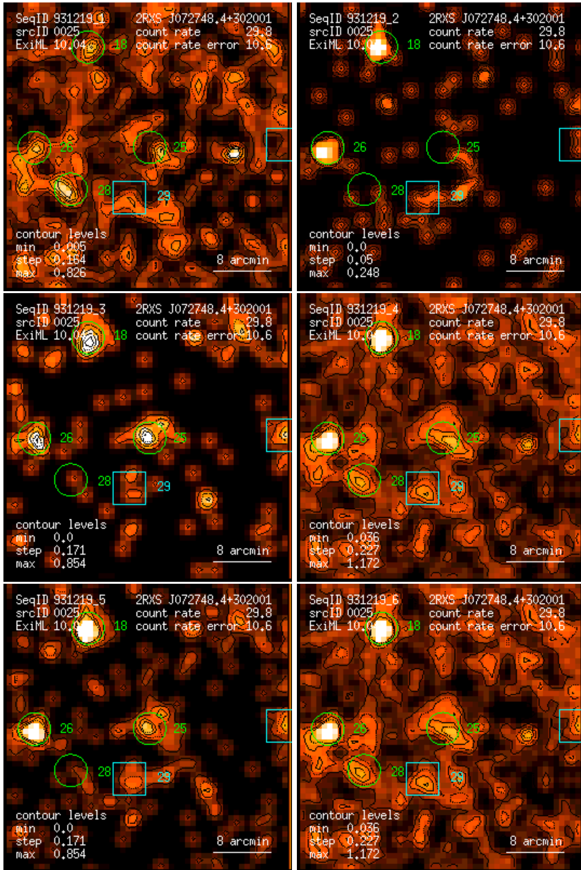
Figure 25: RASS 931219: detection 0025: band rate images, Gaussian filter: (1) PSPC channels 11 – 41, (2) 52 – 90, (3) 91 – 201, (4) 11 – 235, (5) 52 – 201, (6) 11 – 201. Broad band rates in counts/ks. Band rate contour levels in counts/ks/arcmin 2 .
