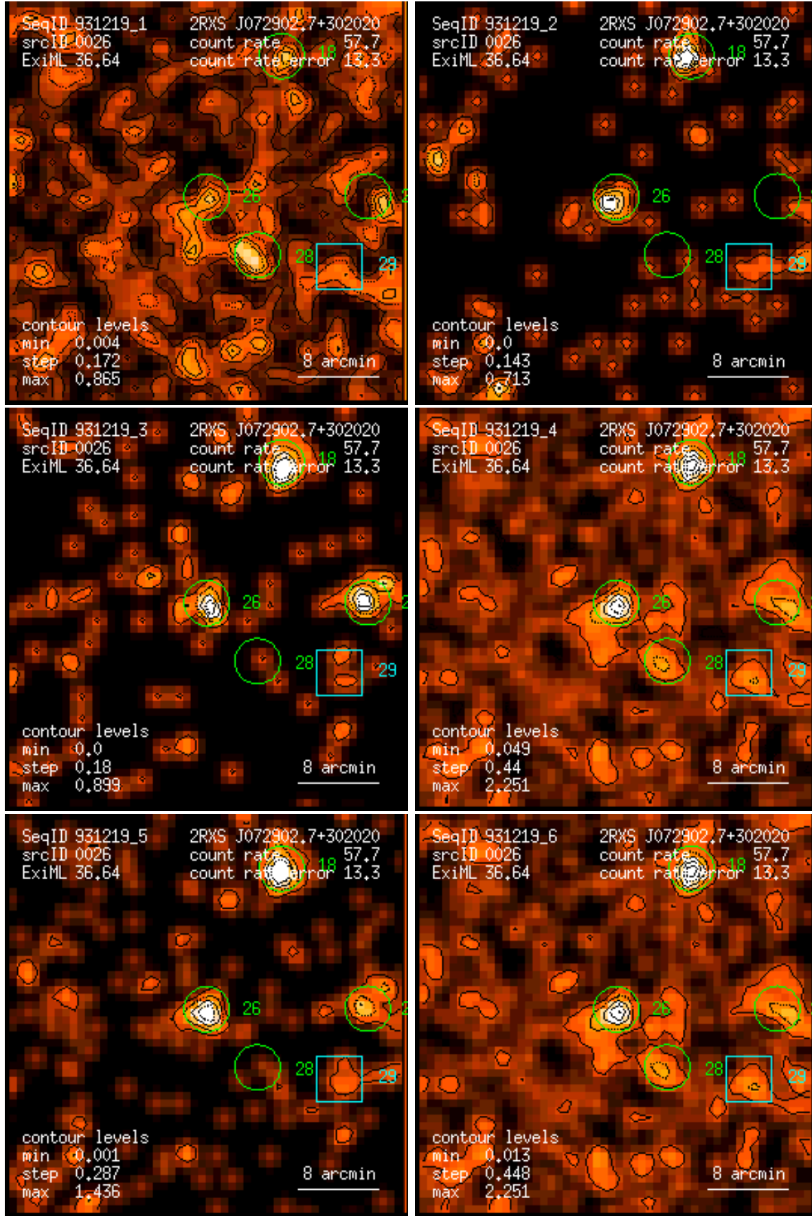
Figure 26: RASS 931219: detection 0026: band rate images, Gaussian filter: (1) PSPC channels 11 – 41, (2) 52 – 90, (3) 91 – 201, (4) 11 – 235, (5) 52 – 201, (6) 11 – 201. Broad band rates in counts/ks. Band rate contour levels in counts/ks/arcmin 2 .
