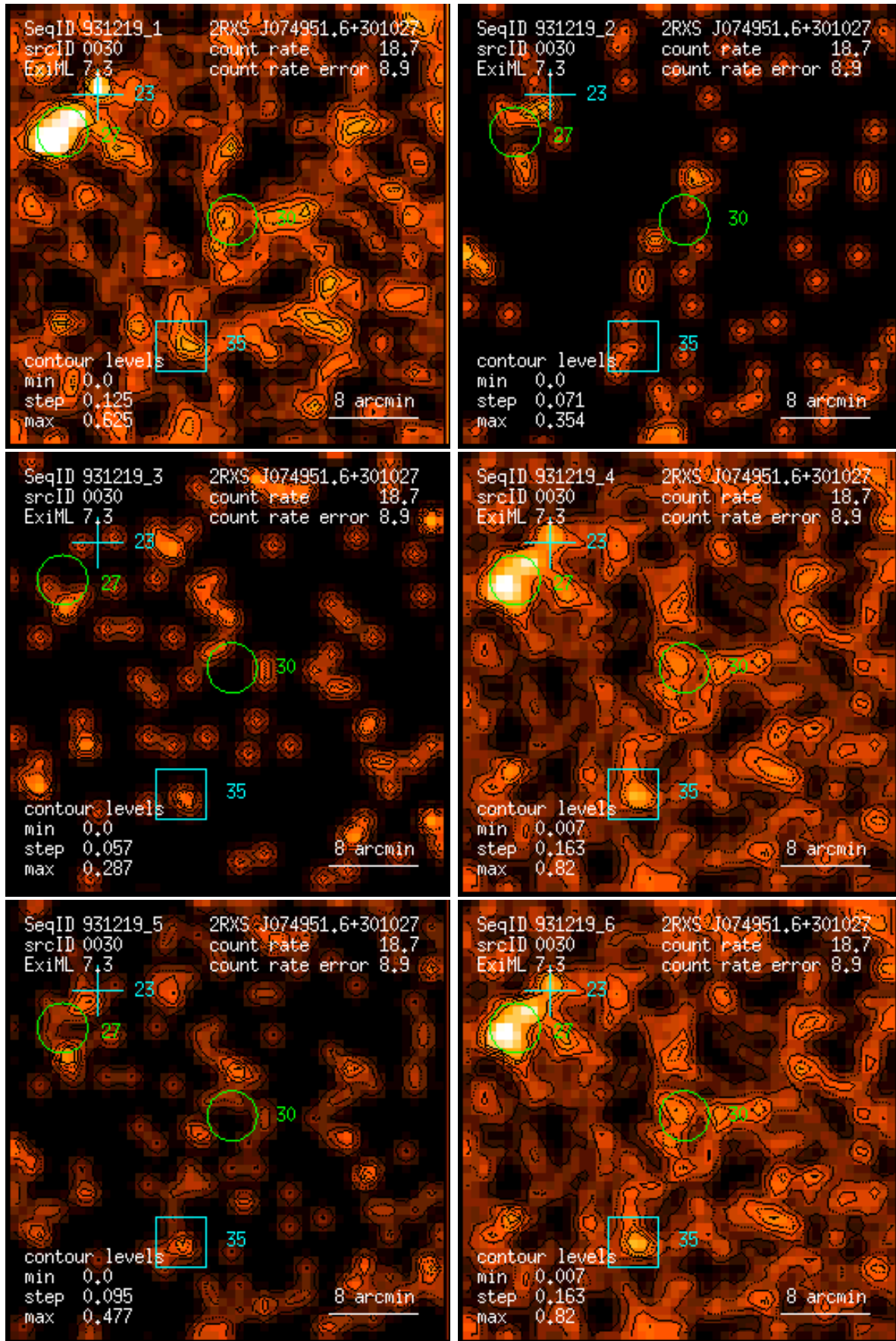
Figure 30: RASS 931219: detection 0030: band rate images, Gaussian filter: (1) PSPC channels 11 – 41, (2) 52 – 90, (3) 91 – 201, (4) 11 – 235, (5) 52 – 201, (6) 11 – 201. Broad band rates in counts/ks. Band rate contour levels in counts/ks/arcmin 2 .
