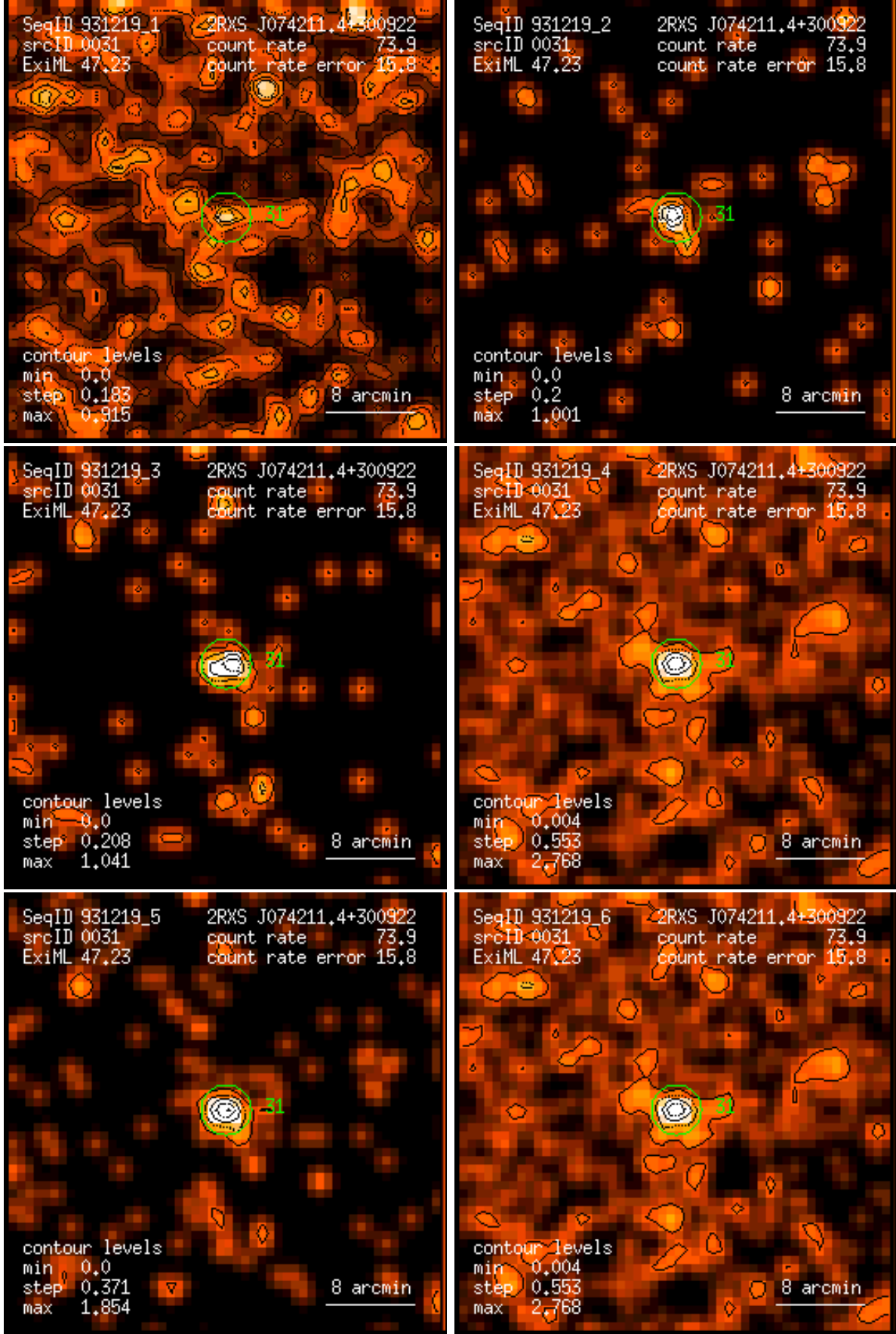
Figure 31: RASS 931219: detection 0031: band rate images, Gaussian filter: (1) PSPC channels 11 – 41, (2) 52 – 90, (3) 91 – 201, (4) 11 – 235, (5) 52 – 201, (6) 11 – 201. Broad band rates in counts/ks. Band rate contour levels in counts/ks/arcmin 2 .
