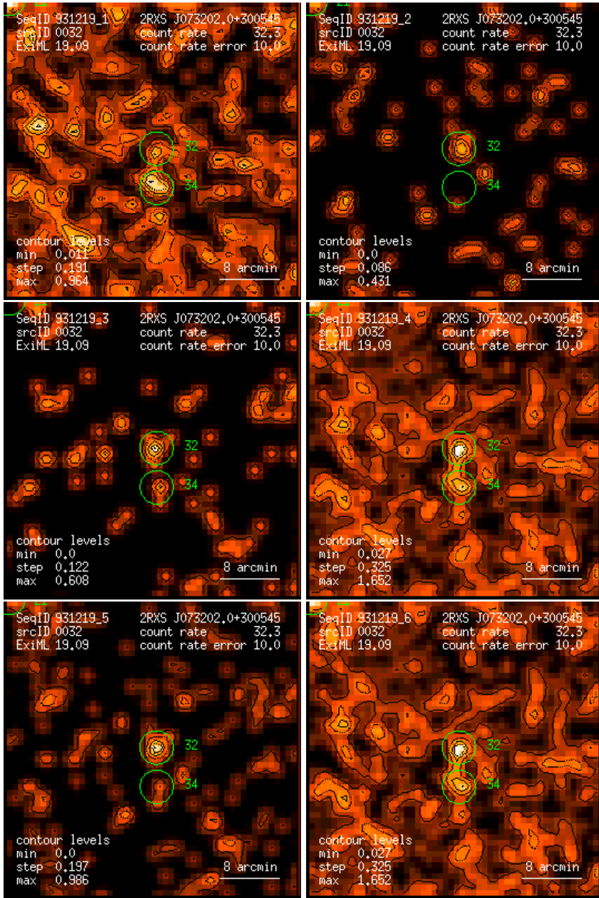
Figure 32: RASS 931219: detection 0032: band rate images, Gaussian filter: (1) PSPC channels 11 – 41, (2) 52 – 90, (3) 91 – 201, (4) 11 – 235, (5) 52 – 201, (6) 11 – 201. Broad band rates in counts/ks. Band rate contour levels in counts/ks/arcmin 2 .
