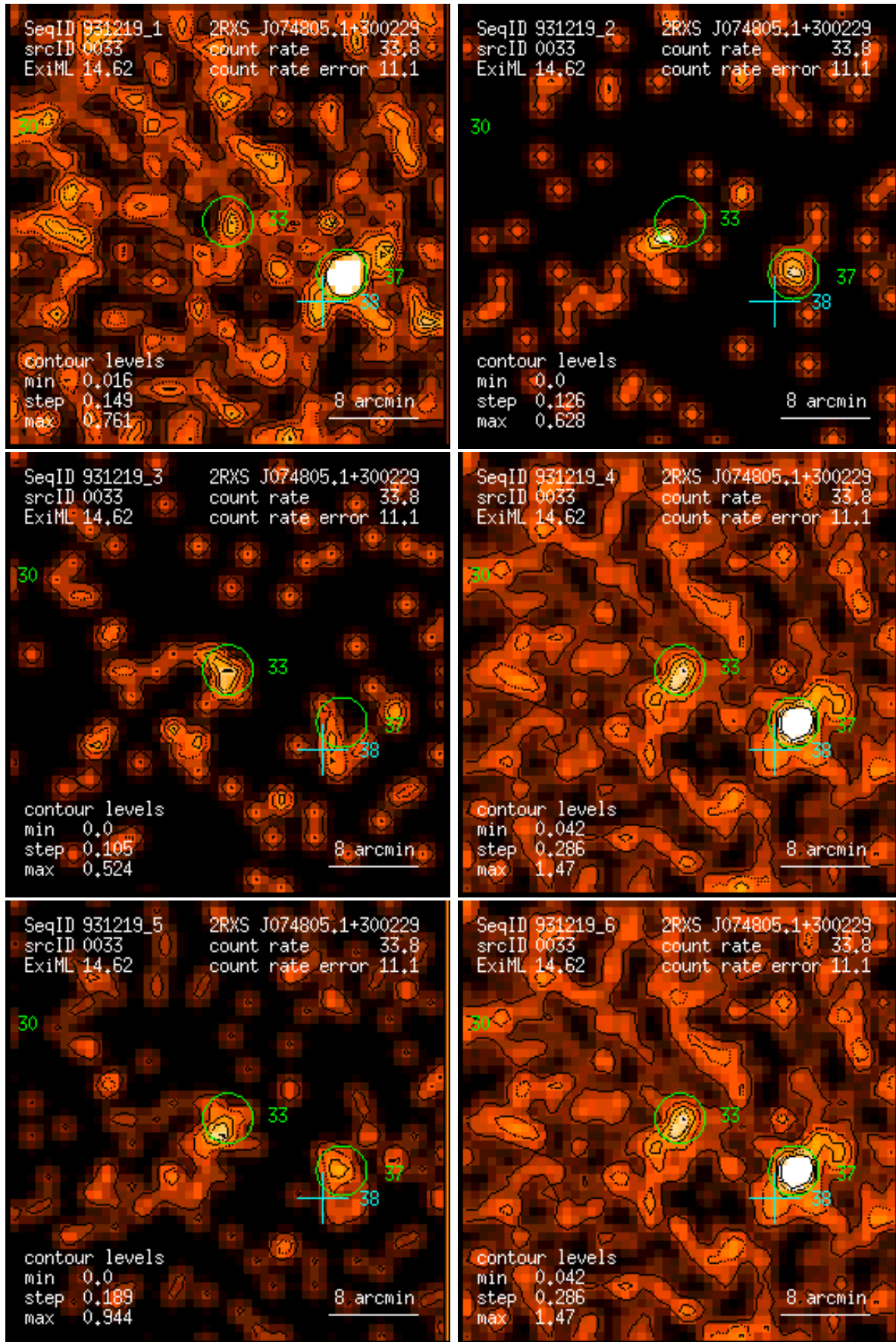
Figure 33: RASS 931219: detection 0033: band rate images, Gaussian filter: (1) PSPC channels 11 – 41, (2) 52 – 90, (3) 91 – 201, (4) 11 – 235, (5) 52 – 201, (6) 11 – 201. Broad band rates in counts/ks. Band rate contour levels in counts/ks/arcmin 2 .
