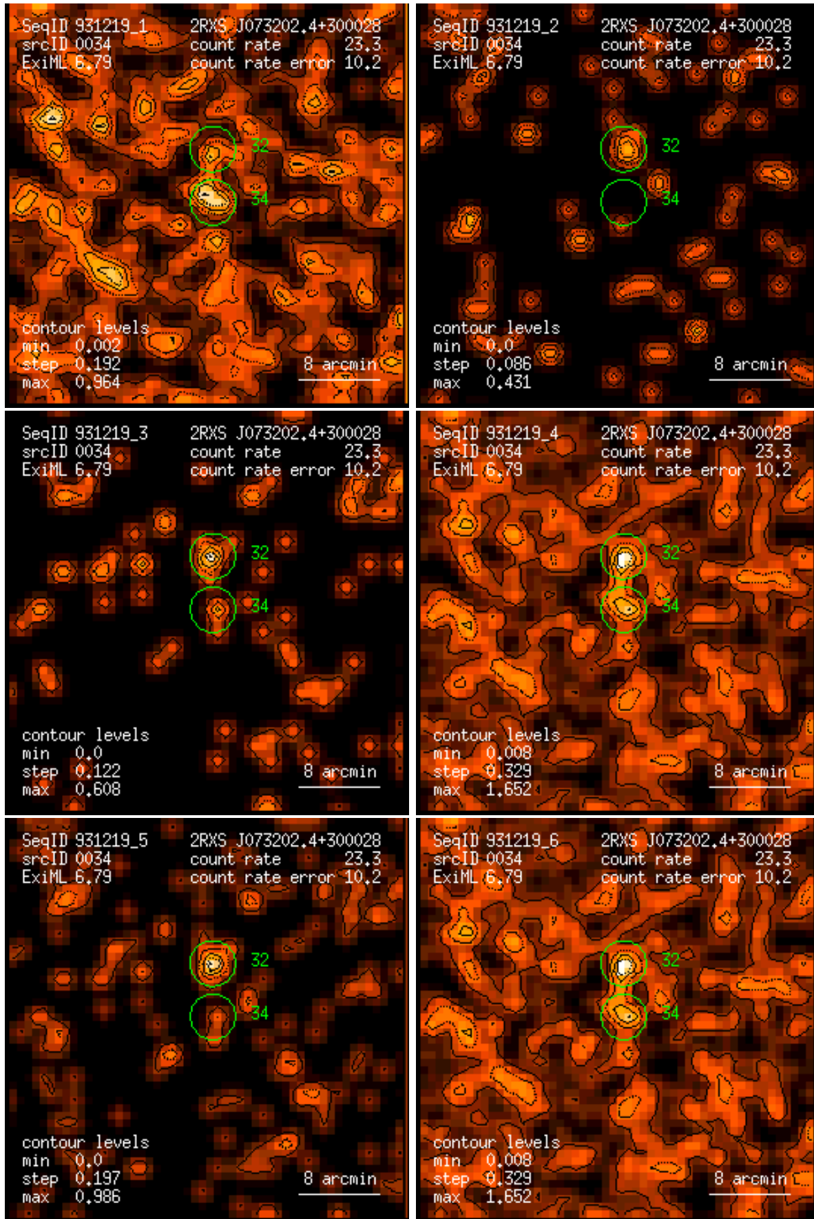
Figure 34: RASS 931219: detection 0034: band rate images, Gaussian filter: (1) PSPC channels 11 – 41, (2) 52 – 90, (3) 91 – 201, (4) 11 – 235, (5) 52 – 201, (6) 11 – 201. Broad band rates in counts/ks. Band rate contour levels in counts/ks/arcmin 2 .
