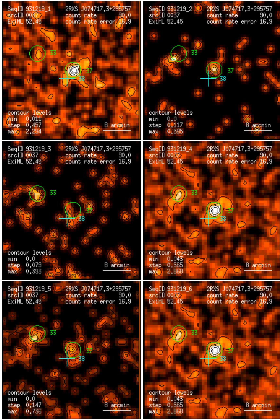
Figure 37: RASS 931219: detection 0037: band rate images, Gaussian filter: (1) PSPC channels 11 – 41, (2) 52 – 90, (3) 91 – 201, (4) 11 – 235, (5) 52 – 201, (6) 11 – 201. Broad band rates in counts/ks. Band rate contour levels in counts/ks/arcmin 2 .
