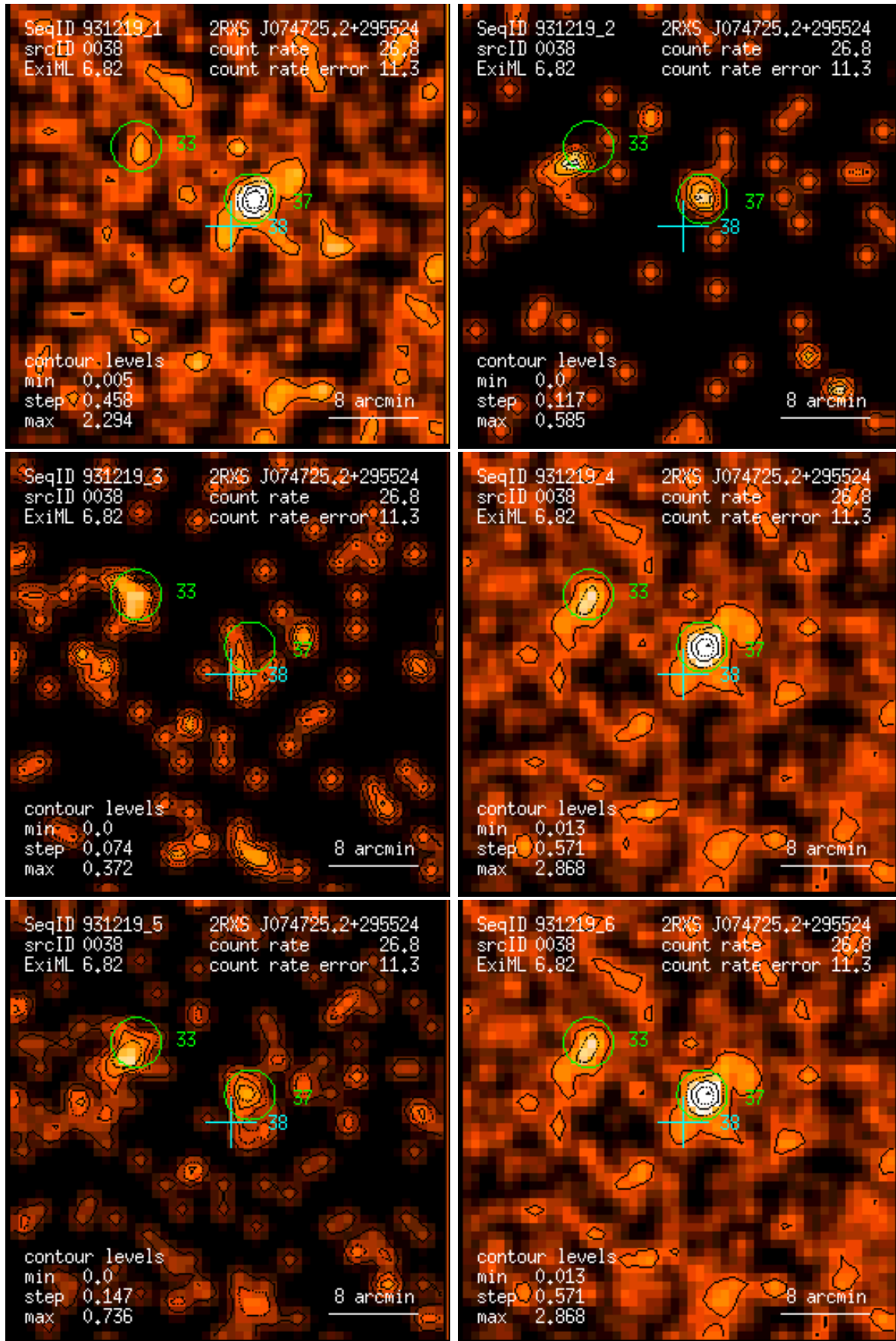
Figure 38: RASS 931219: detection 0038: band rate images, Gaussian filter: (1) PSPC channels 11 – 41, (2) 52 – 90, (3) 91 – 201, (4) 11 – 235, (5) 52 – 201, (6) 11 – 201. Broad band rates in counts/ks. Band rate contour levels in counts/ks/arcmin 2 .
