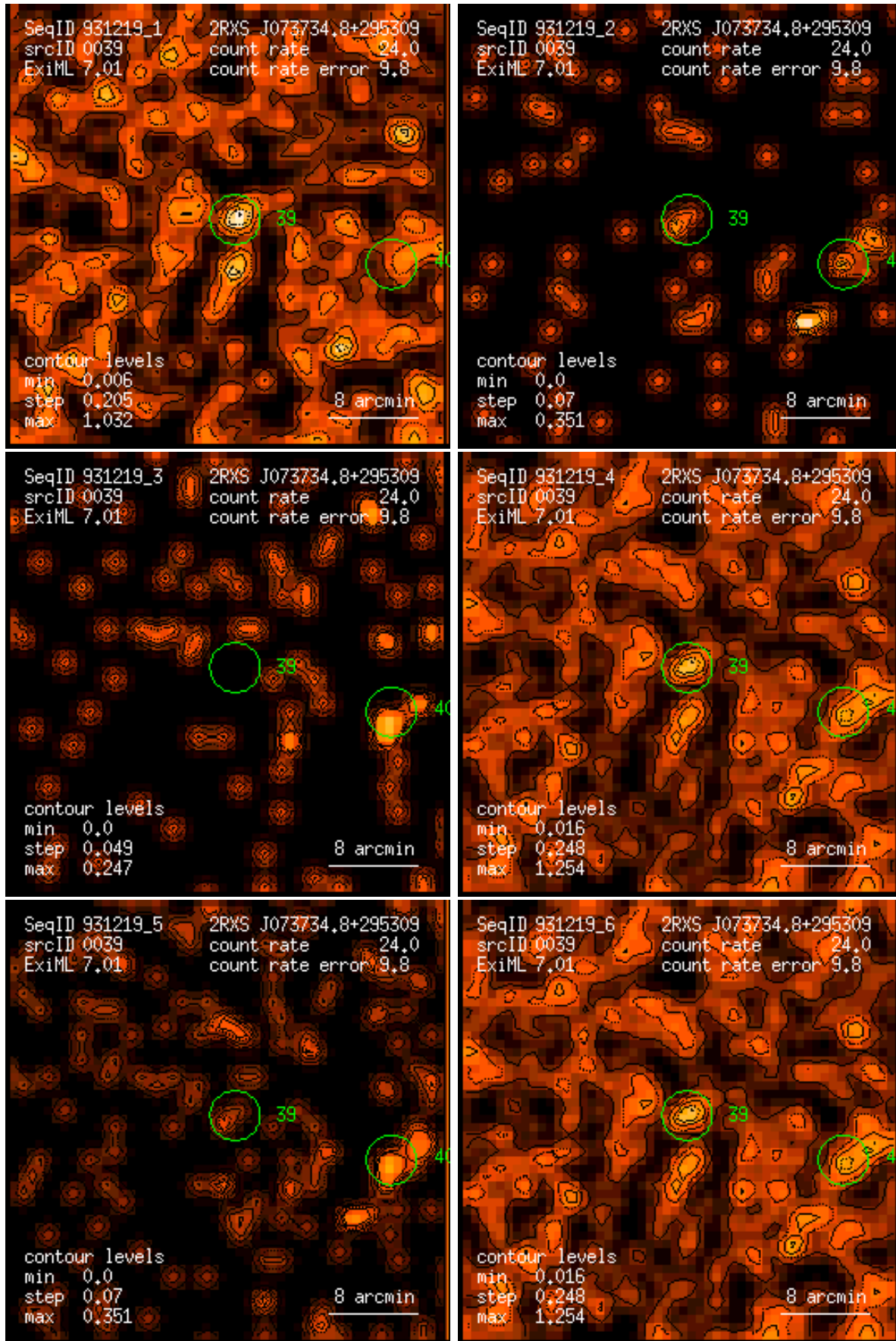
Figure 39: RASS 931219: detection 0039: band rate images, Gaussian filter: (1) PSPC channels 11 – 41, (2) 52 – 90, (3) 91 – 201, (4) 11 – 235, (5) 52 – 201, (6) 11 – 201. Broad band rates in counts/ks. Band rate contour levels in counts/ks/arcmin 2 .
