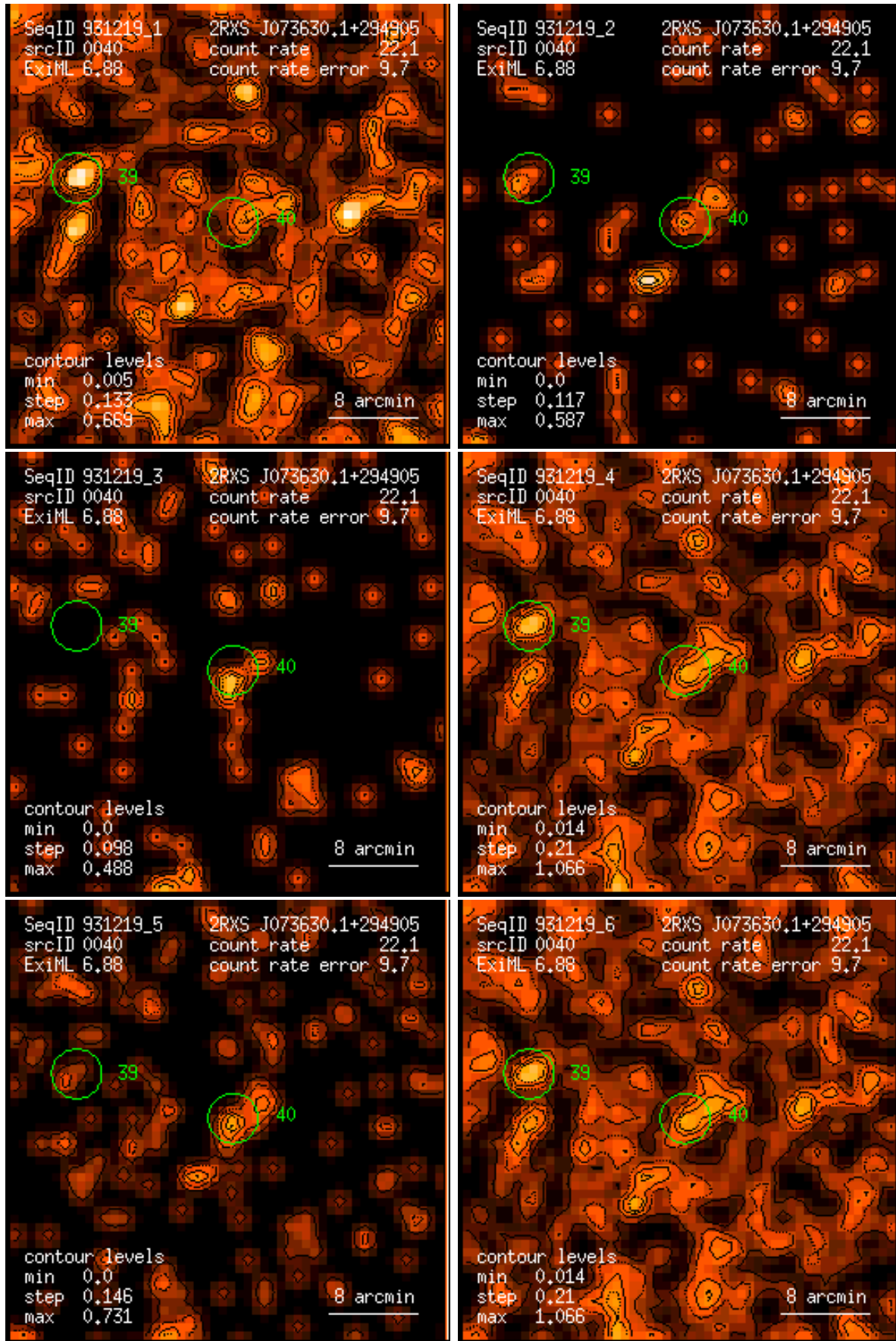
Figure 40: RASS 931219: detection 0040: band rate images, Gaussian filter: (1) PSPC channels 11 – 41, (2) 52 – 90, (3) 91 – 201, (4) 11 – 235, (5) 52 – 201, (6) 11 – 201. Broad band rates in counts/ks. Band rate contour levels in counts/ks/arcmin 2 .
