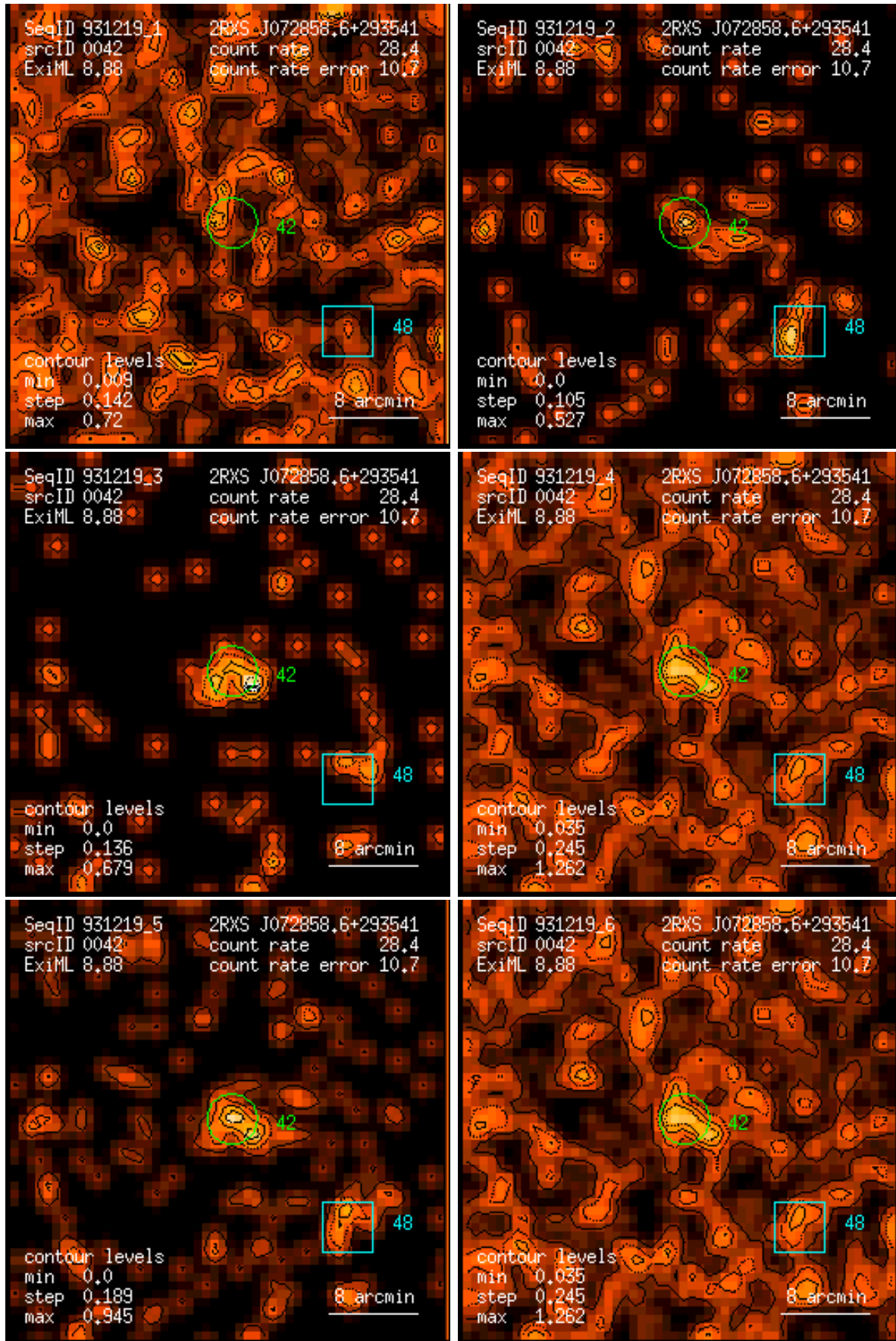
Figure 42: RASS 931219: detection 0042: band rate images, Gaussian filter: (1) PSPC channels 11 – 41, (2) 52 – 90, (3) 91 – 201, (4) 11 – 235, (5) 52 – 201, (6) 11 – 201. Broad band rates in counts/ks. Band rate contour levels in counts/ks/arcmin 2 .
