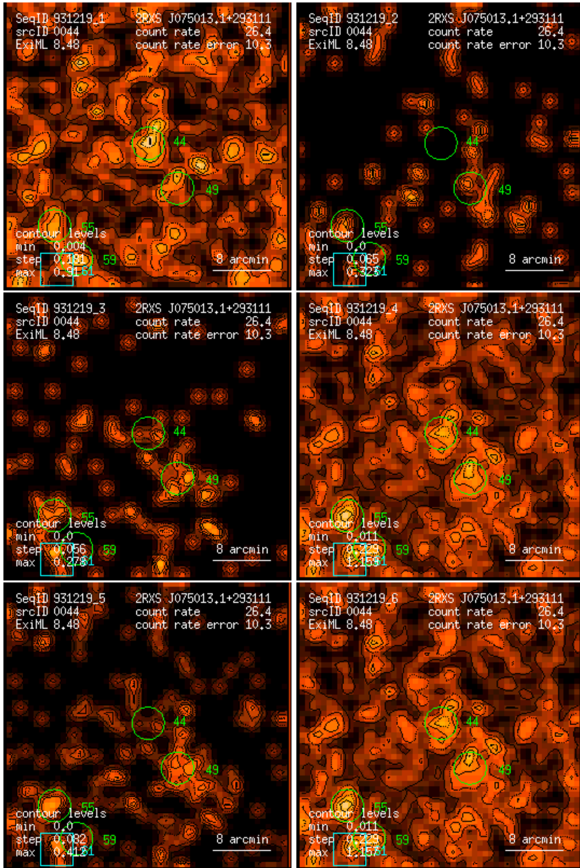
Figure 44: RASS 931219: detection 0044: band rate images, Gaussian filter: (1) PSPC channels 11 – 41, (2) 52 – 90, (3) 91 – 201, (4) 11 – 235, (5) 52 – 201, (6) 11 – 201. Broad band rates in counts/ks. Band rate contour levels in counts/ks/arcmin 2 .
