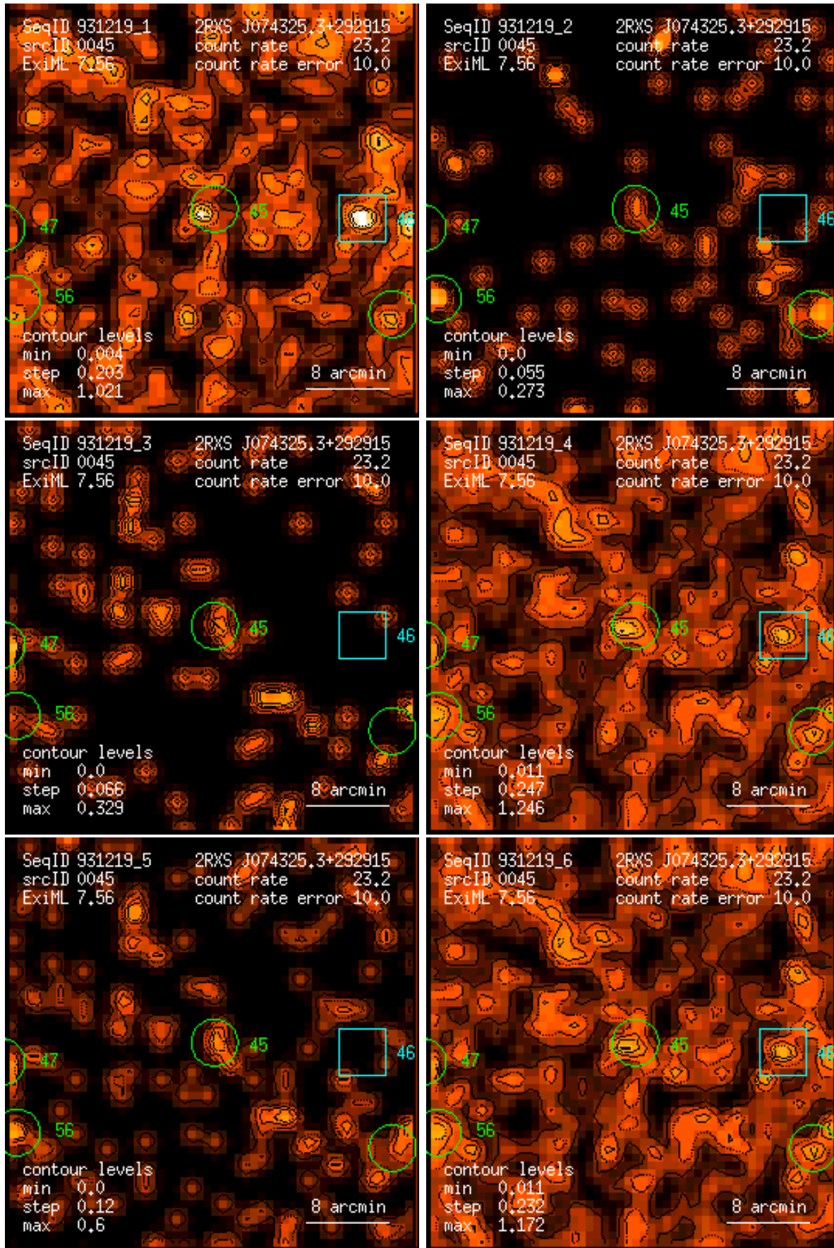
Figure 45: RASS 931219: detection 0045: band rate images, Gaussian filter: (1) PSPC channels 11 – 41, (2) 52 – 90, (3) 91 – 201, (4) 11 – 235, (5) 52 – 201, (6) 11 – 201. Broad band rates in counts/ks. Band rate contour levels in counts/ks/arcmin 2 .
