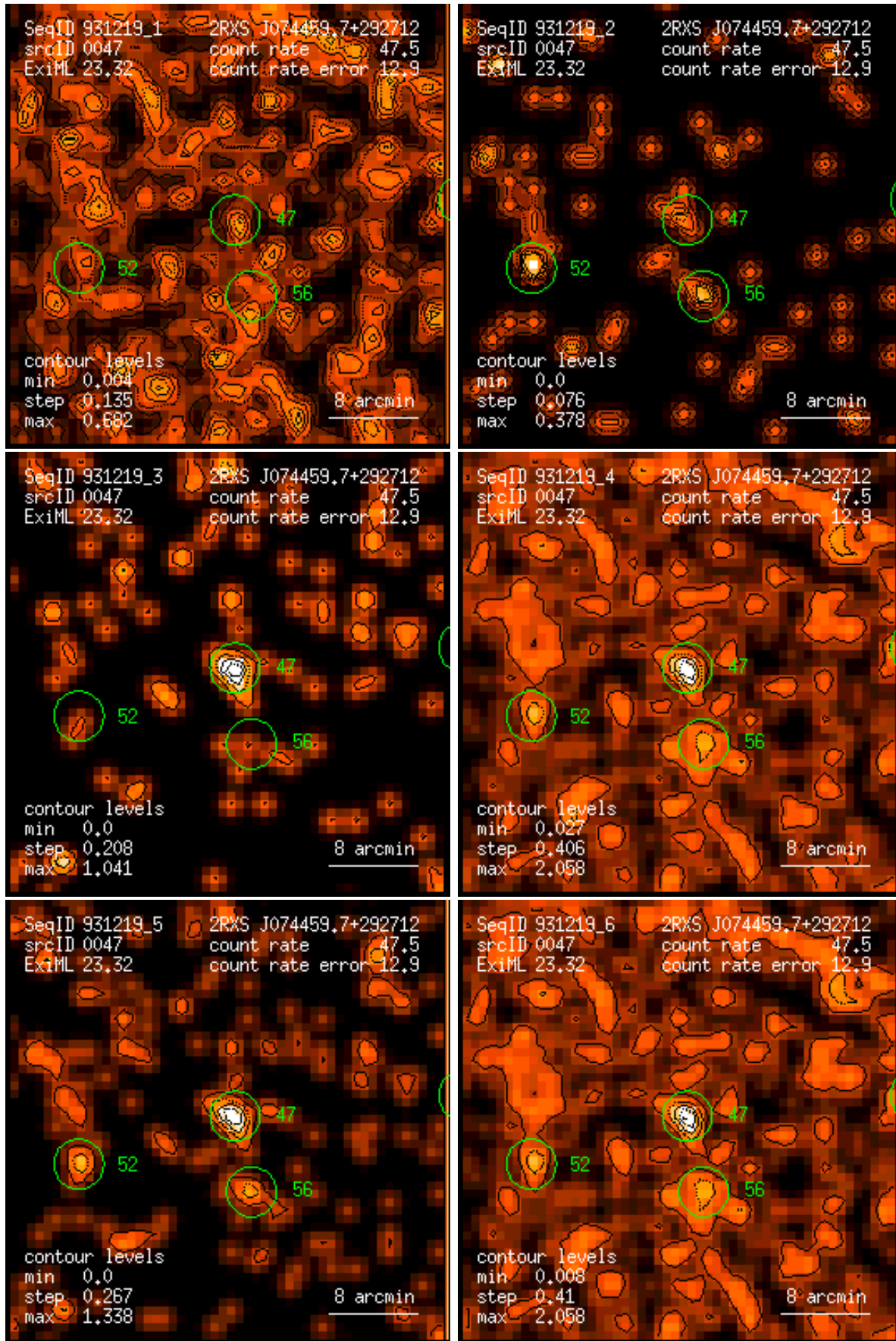
Figure 47: RASS 931219: detection 0047: band rate images, Gaussian filter: (1) PSPC channels 11 – 41, (2) 52 – 90, (3) 91 – 201, (4) 11 – 235, (5) 52 – 201, (6) 11 – 201. Broad band rates in counts/ks. Band rate contour levels in counts/ks/arcmin 2 .
