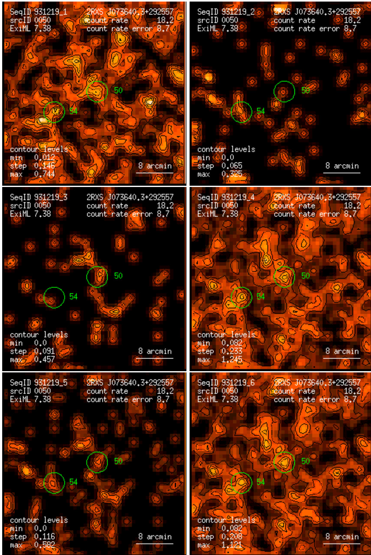
Figure 50: RASS 931219: detection 0050: band rate images, Gaussian filter: (1) PSPC channels 11 – 41, (2) 52 – 90, (3) 91 – 201, (4) 11 – 235, (5) 52 – 201, (6) 11 – 201. Broad band rates in counts/ks. Band rate contour levels in counts/ks/arcmin 2 .
