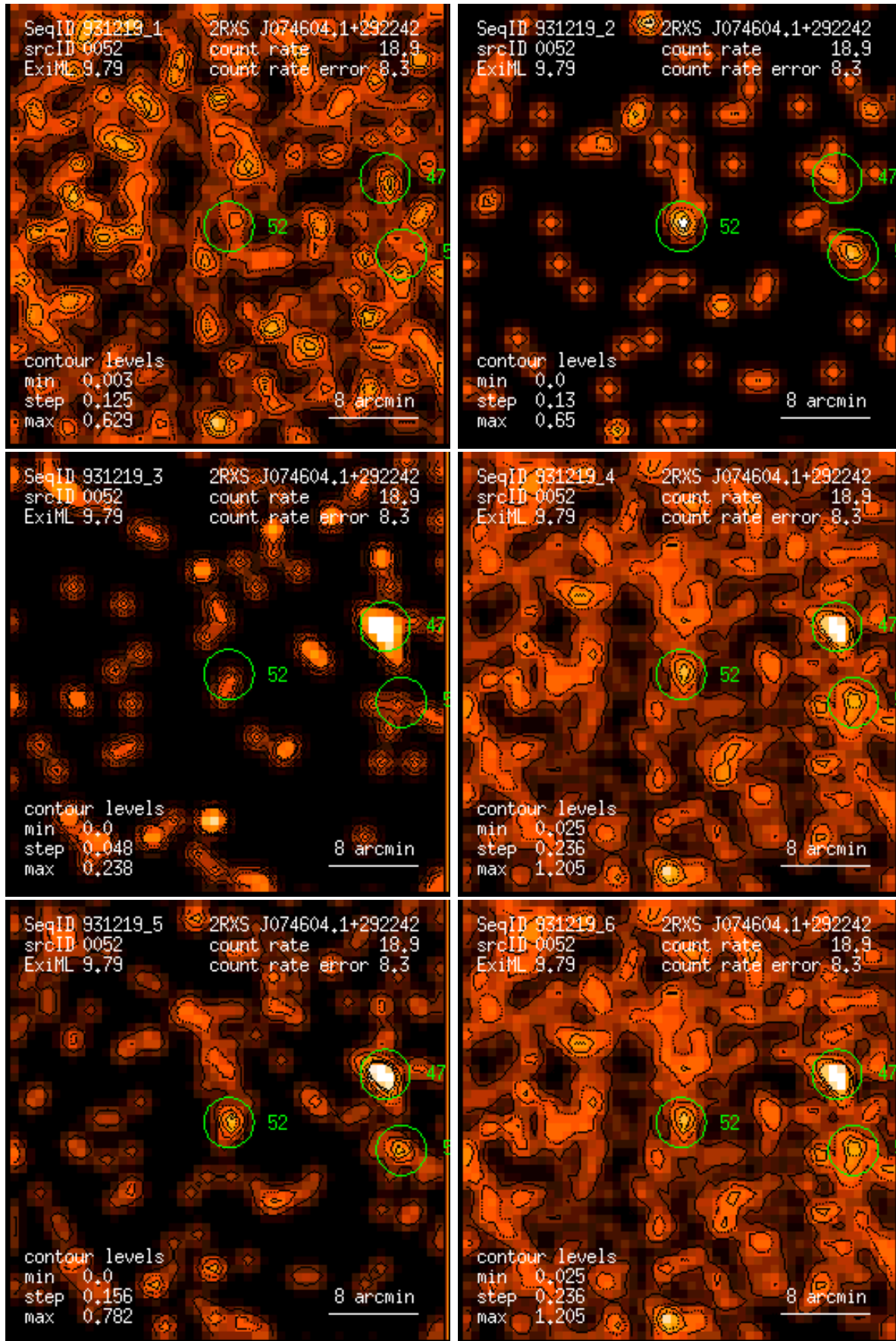
Figure 52: RASS 931219: detection 0052: band rate images, Gaussian filter: (1) PSPC channels 11 – 41, (2) 52 – 90, (3) 91 – 201, (4) 11 – 235, (5) 52 – 201, (6) 11 – 201. Broad band rates in counts/ks. Band rate contour levels in counts/ks/arcmin 2 .
