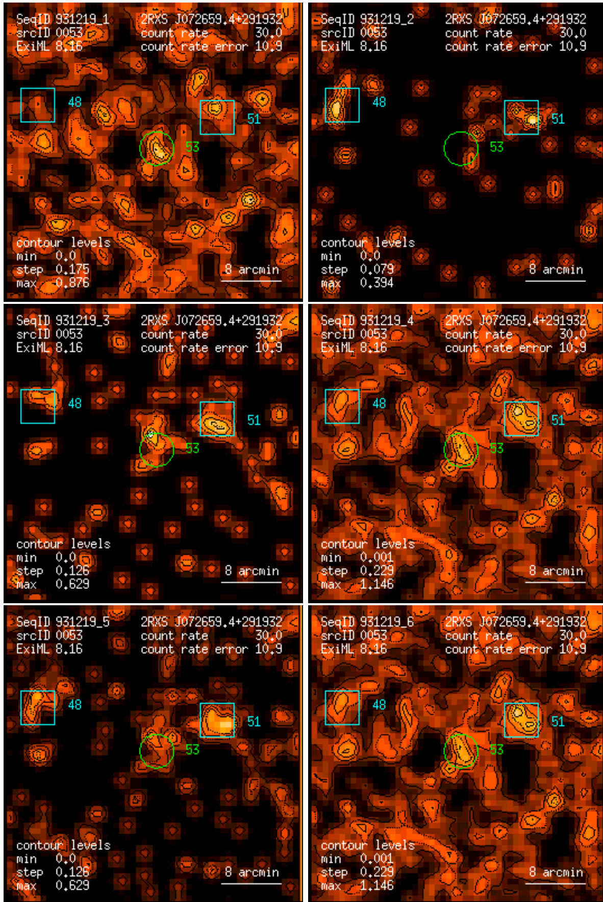
Figure 53: RASS 931219: detection 0053: band rate images, Gaussian filter: (1) PSPC channels 11 – 41, (2) 52 – 90, (3) 91 – 201, (4) 11 – 235, (5) 52 – 201, (6) 11 – 201. Broad band rates in counts/ks. Band rate contour levels in counts/ks/arcmin 2 .
