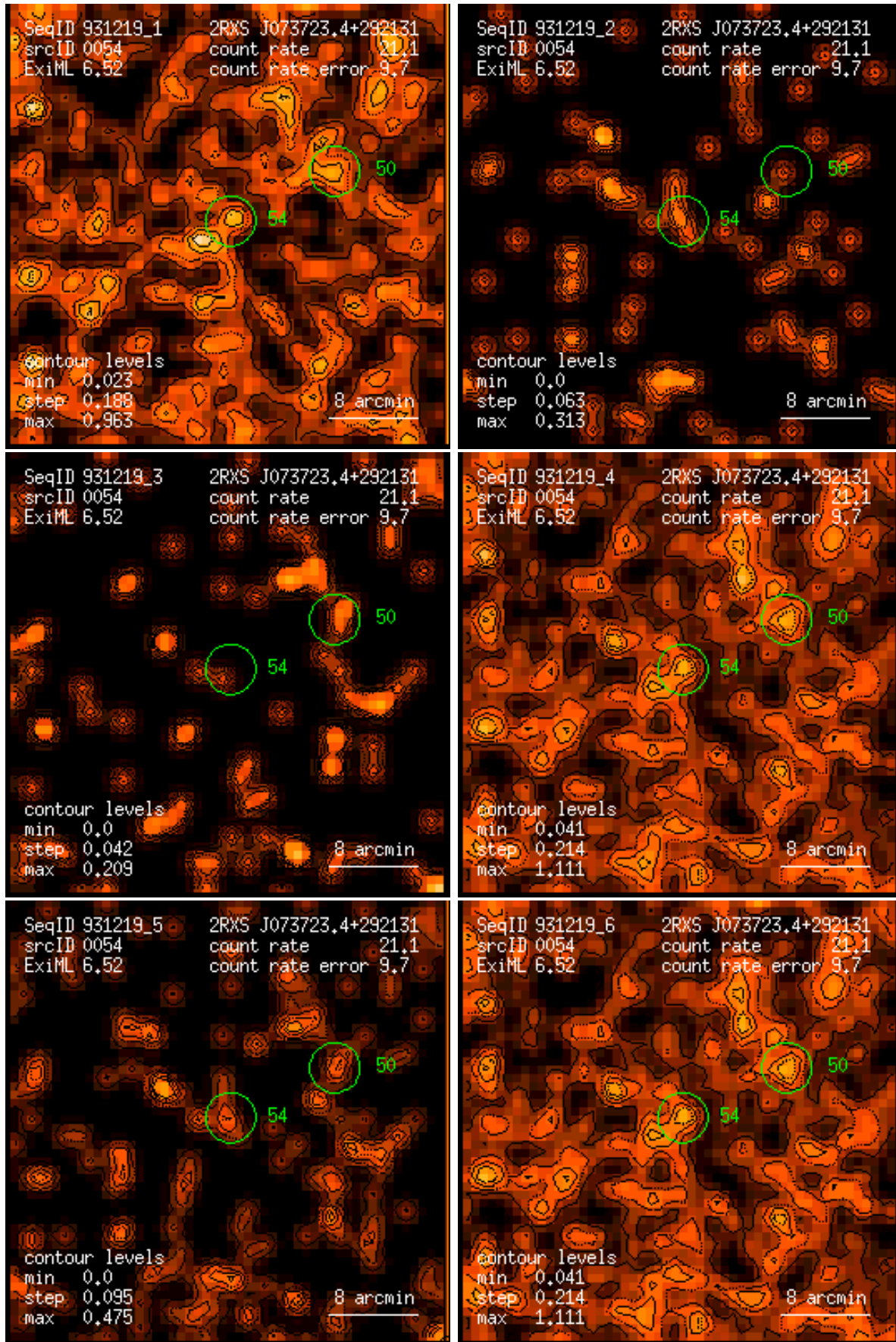
Figure 54: RASS 931219: detection 0054: band rate images, Gaussian filter: (1) PSPC channels 11 – 41, (2) 52 – 90, (3) 91 – 201, (4) 11 – 235, (5) 52 – 201, (6) 11 – 201. Broad band rates in counts/ks. Band rate contour levels in counts/ks/arcmin 2 .
