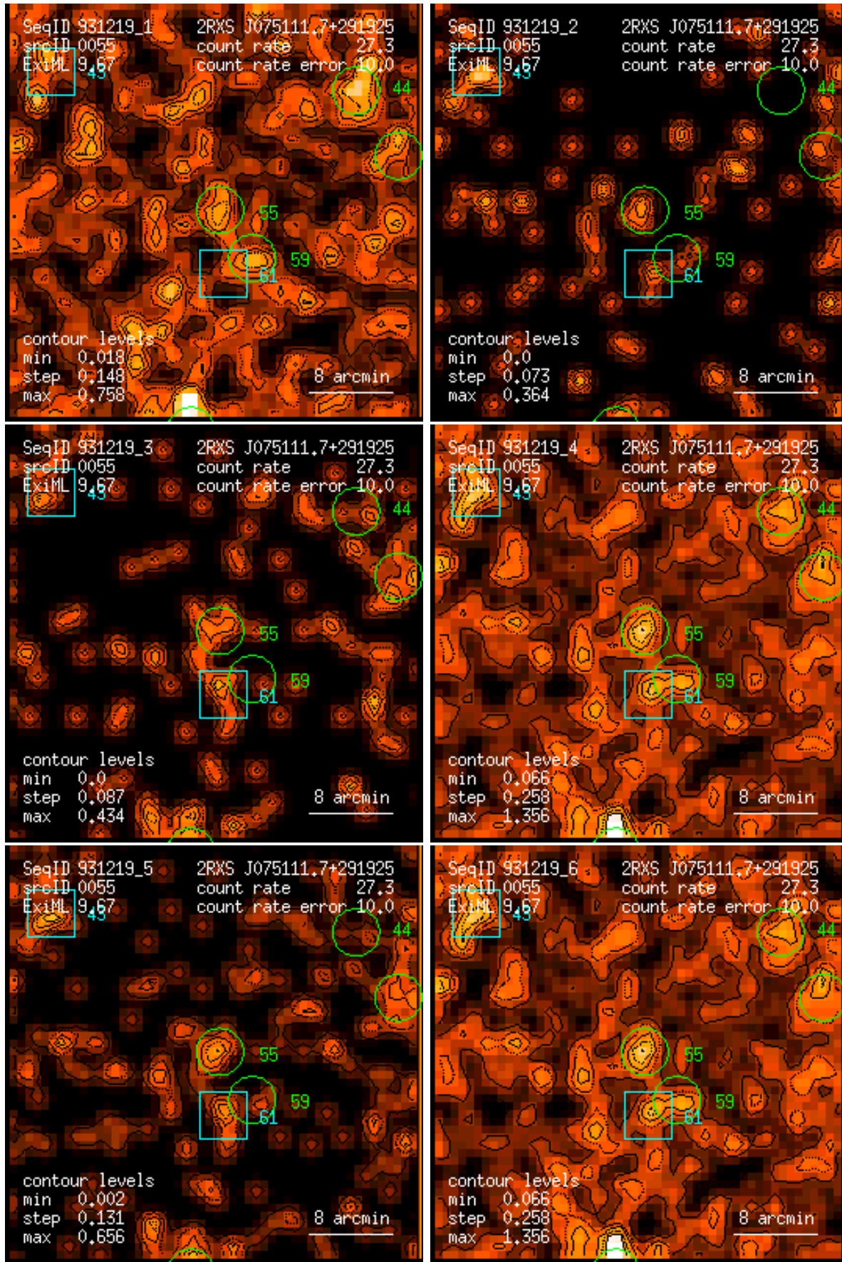
Figure 55: RASS 931219: detection 0055: band rate images, Gaussian filter: (1) PSPC channels 11 – 41, (2) 52 – 90, (3) 91 – 201, (4) 11 – 235, (5) 52 – 201, (6) 11 – 201. Broad band rates in counts/ks. Band rate contour levels in counts/ks/arcmin 2 .
