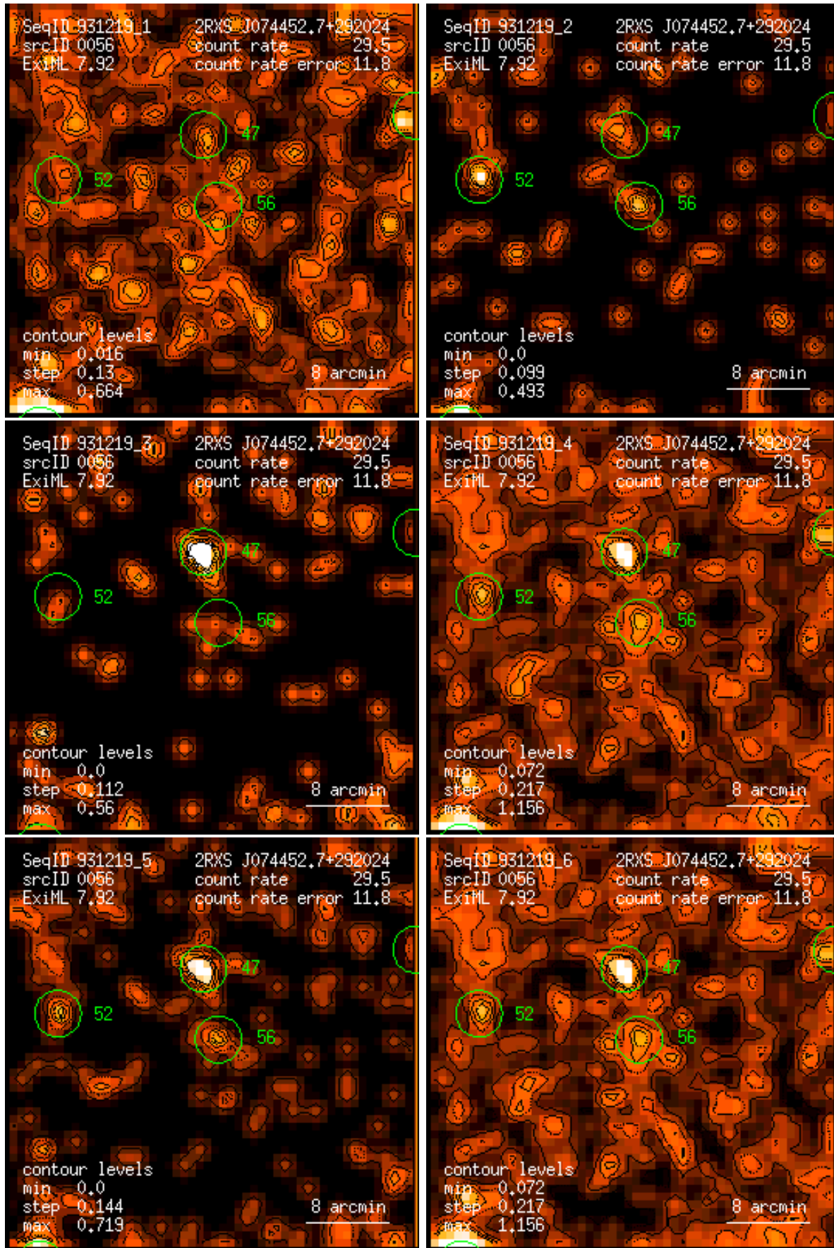
Figure 56: RASS 931219: detection 0056: band rate images, Gaussian filter: (1) PSPC channels 11 – 41, (2) 52 – 90, (3) 91 – 201, (4) 11 – 235, (5) 52 – 201, (6) 11 – 201. Broad band rates in counts/ks. Band rate contour levels in counts/ks/arcmin 2 .
