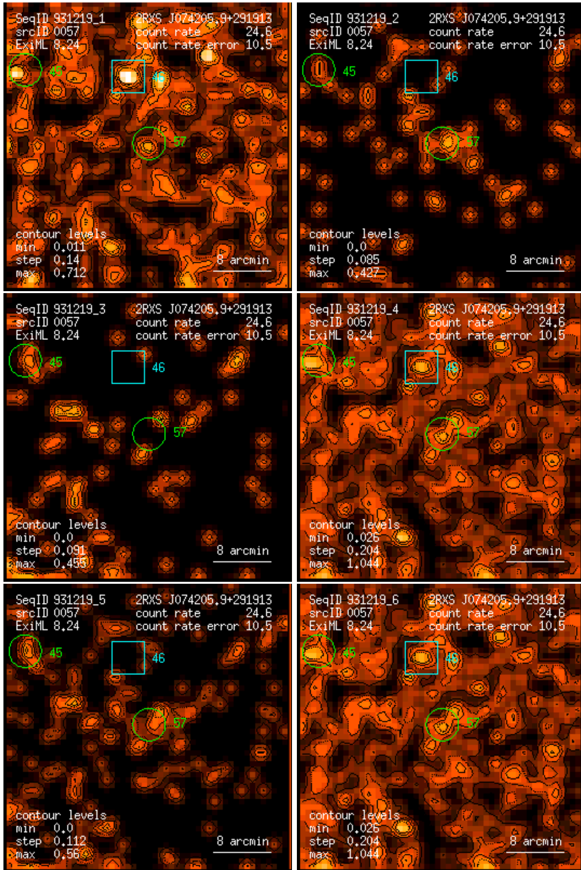
Figure 57: RASS 931219: detection 0057: band rate images, Gaussian filter: (1) PSPC channels 11 – 41, (2) 52 – 90, (3) 91 – 201, (4) 11 – 235, (5) 52 – 201, (6) 11 – 201. Broad band rates in counts/ks. Band rate contour levels in counts/ks/arcmin 2 .
