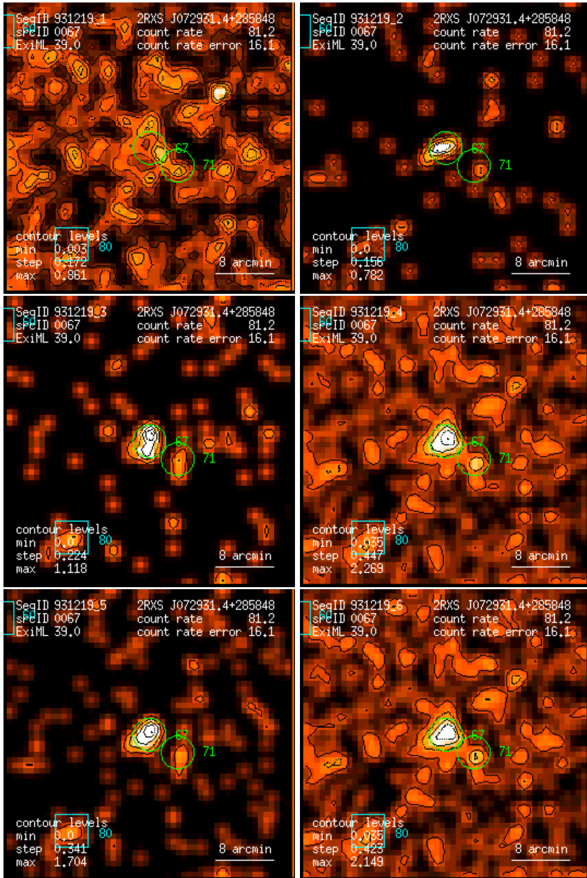
Figure 67: RASS 931219: detection 0067: band rate images, Gaussian filter: (1) PSPC channels 11 – 41, (2) 52 – 90, (3) 91 – 201, (4) 11 – 235, (5) 52 – 201, (6) 11 – 201. Broad band rates in counts/ks. Band rate contour levels in counts/ks/arcmin 2 .
