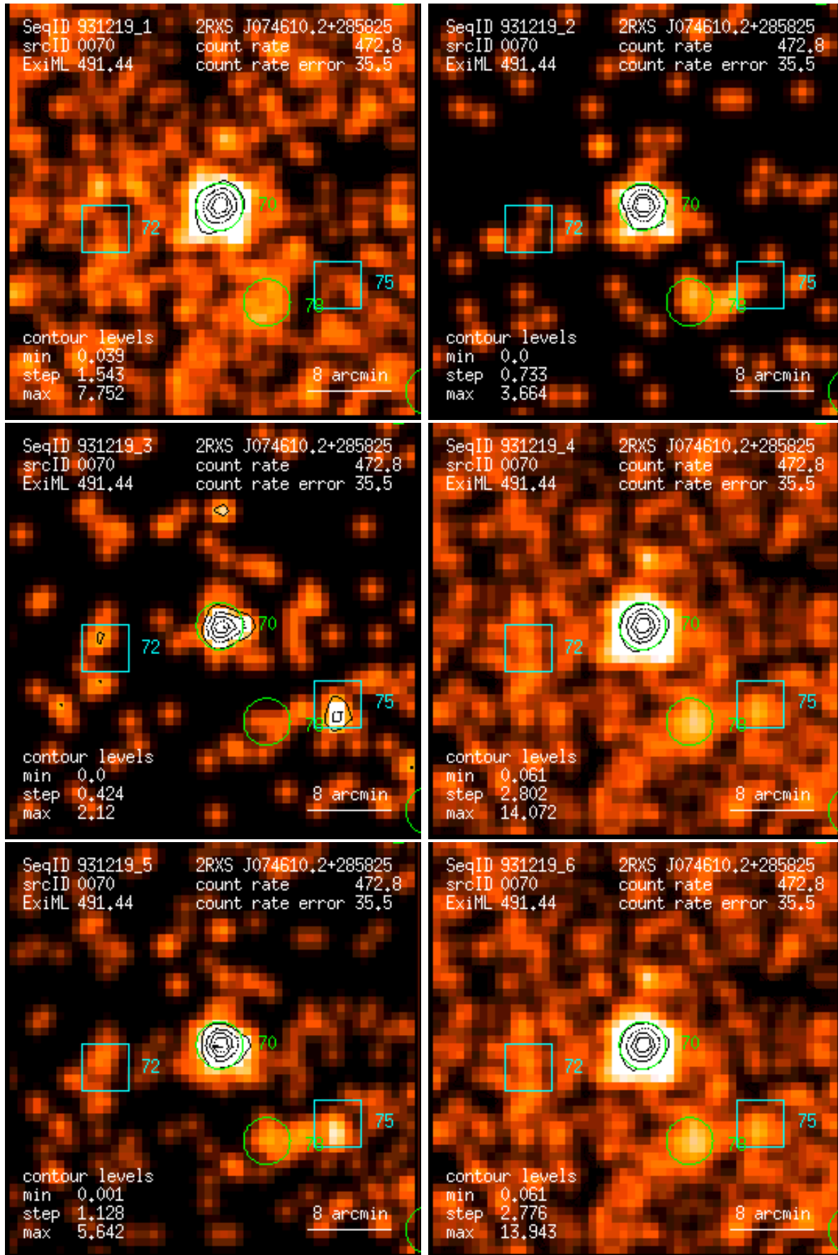
Figure 70: RASS 931219: detection 0070: band rate images, Gaussian filter: (1) PSPC channels 11 – 41, (2) 52 – 90, (3) 91 – 201, (4) 11 – 235, (5) 52 – 201, (6) 11 – 201. Broad band rates in counts/ks. Band rate contour levels in counts/ks/arcmin 2 .
