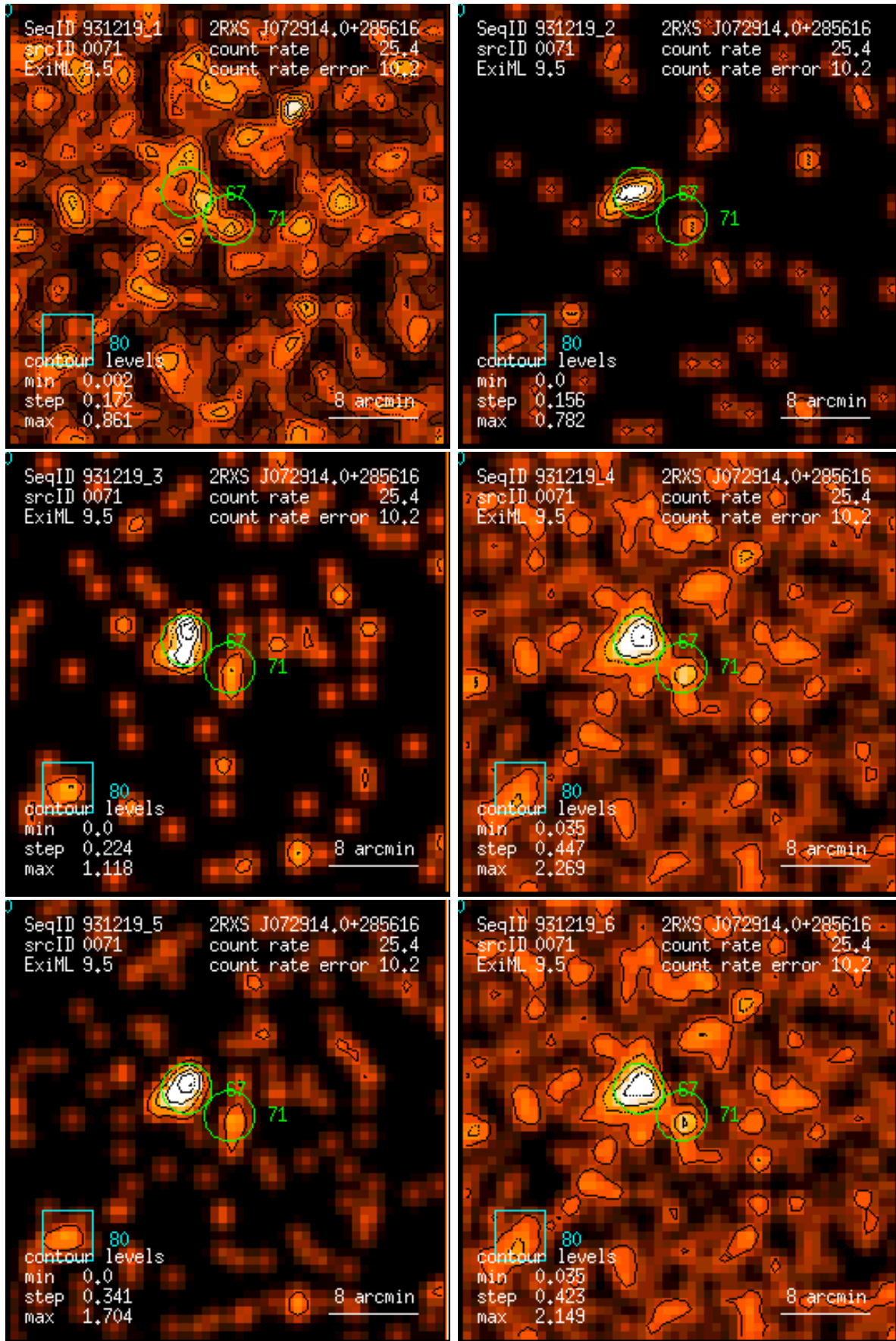
Figure 71: RASS 931219: detection 0071: band rate images, Gaussian filter: (1) PSPC channels 11 – 41, (2) 52 – 90, (3) 91 – 201, (4) 11 – 235, (5) 52 – 201, (6) 11 – 201. Broad band rates in counts/ks. Band rate contour levels in counts/ks/arcmin 2 .
