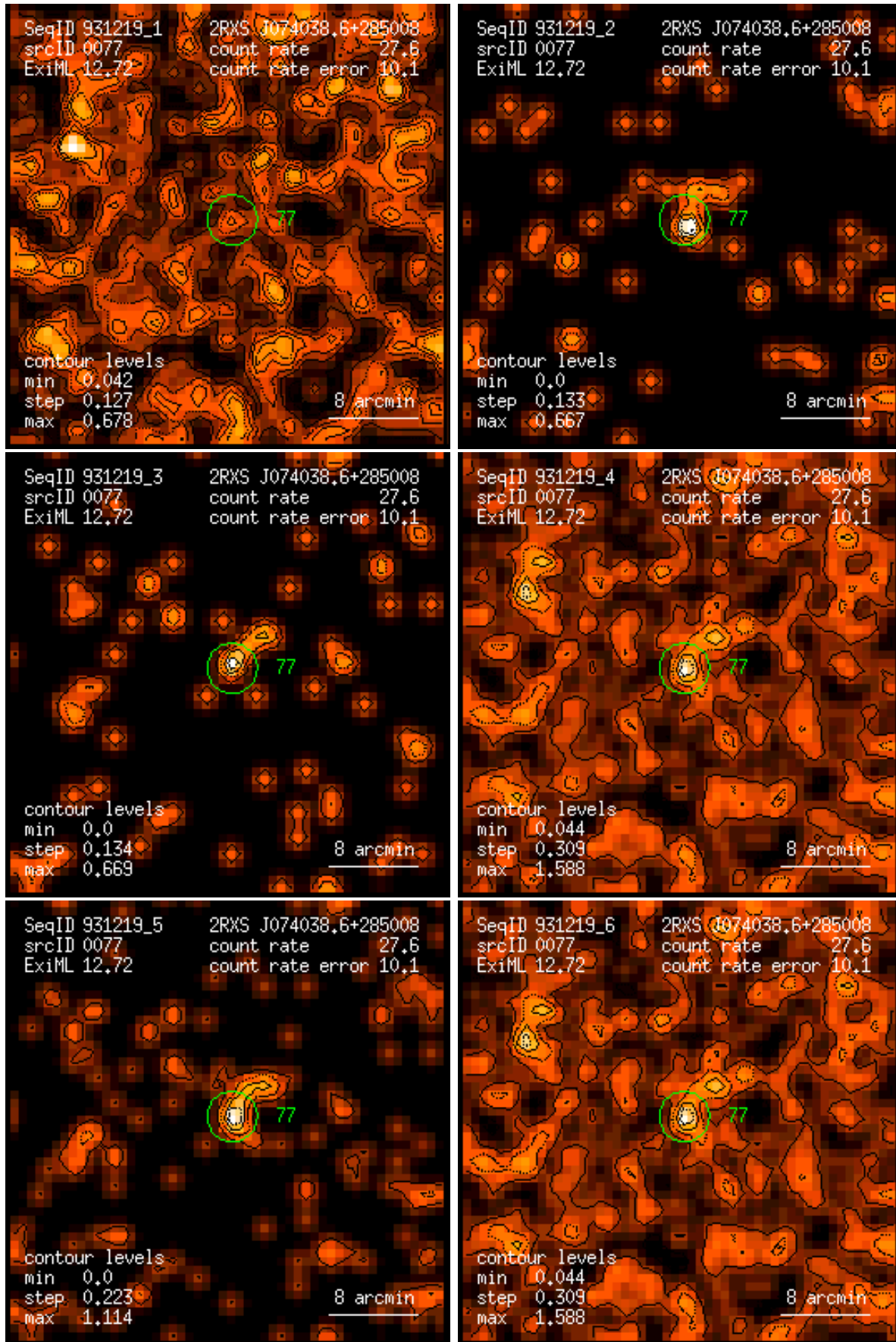
Figure 77: RASS 931219: detection 0077: band rate images, Gaussian filter: (1) PSPC channels 11 – 41, (2) 52 – 90, (3) 91 – 201, (4) 11 – 235, (5) 52 – 201, (6) 11 – 201. Broad band rates in counts/ks. Band rate contour levels in counts/ks/arcmin 2 .
