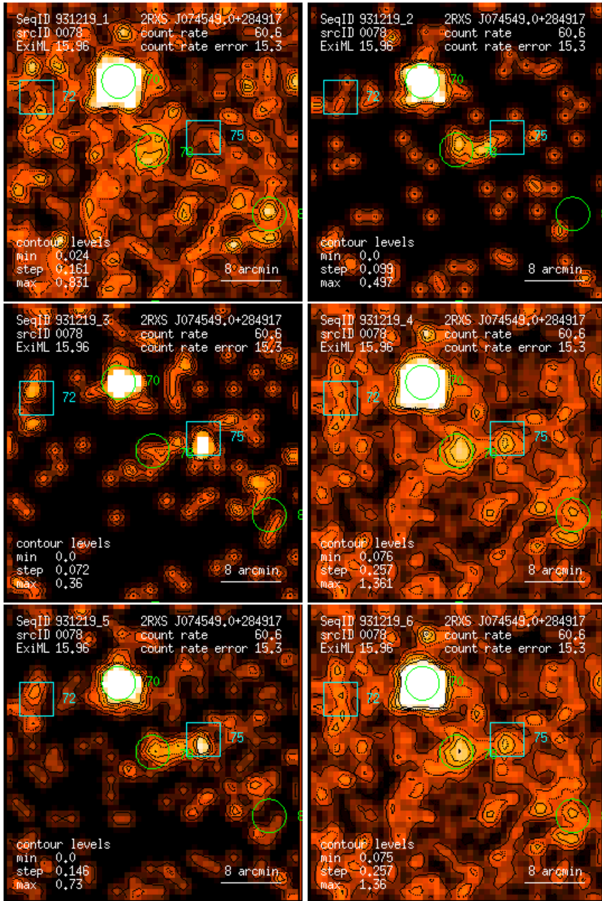
Figure 78: RASS 931219: detection 0078: band rate images, Gaussian filter: (1) PSPC channels 11 – 41, (2) 52 – 90, (3) 91 – 201, (4) 11 – 235, (5) 52 – 201, (6) 11 – 201. Broad band rates in counts/ks. Band rate contour levels in counts/ks/arcmin 2 .
