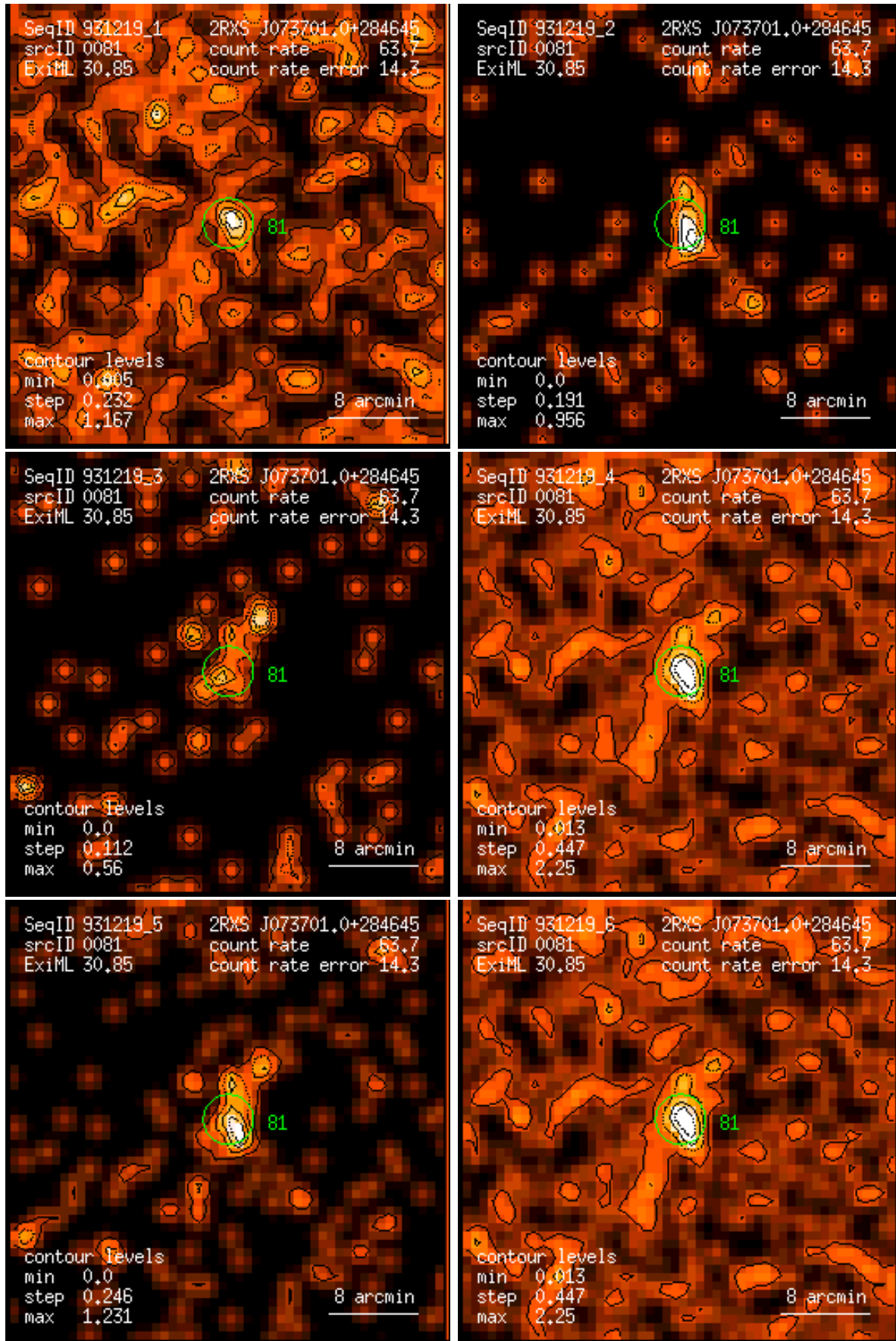
Figure 81: RASS 931219: detection 0081: band rate images, Gaussian filter: (1) PSPC channels 11 – 41, (2) 52 – 90, (3) 91 – 201, (4) 11 – 235, (5) 52 – 201, (6) 11 – 201. Broad band rates in counts/ks. Band rate contour levels in counts/ks/arcmin 2 .
