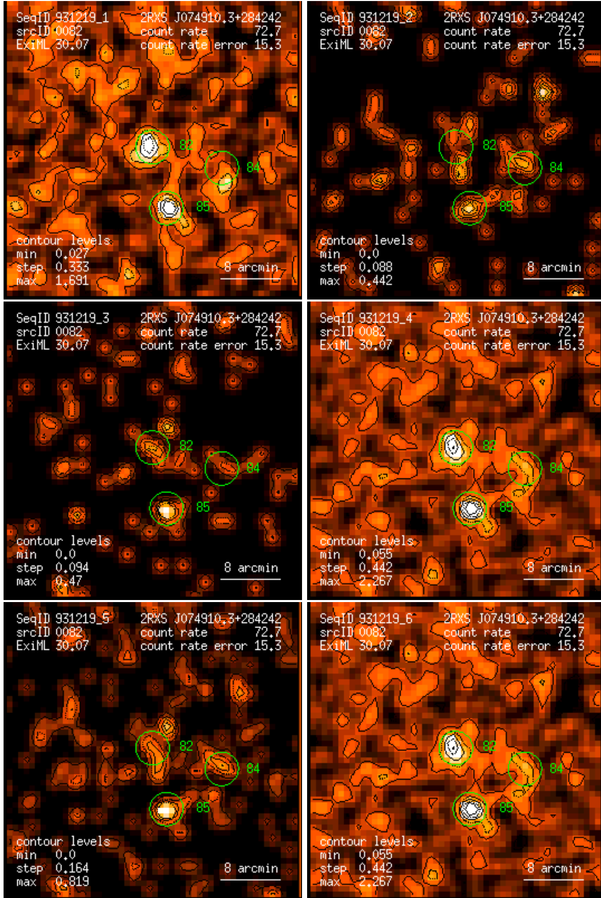
Figure 82: RASS 931219: detection 0082: band rate images, Gaussian filter: (1) PSPC channels 11 – 41, (2) 52 – 90, (3) 91 – 201, (4) 11 – 235, (5) 52 – 201, (6) 11 – 201. Broad band rates in counts/ks. Band rate contour levels in counts/ks/arcmin 2 .
