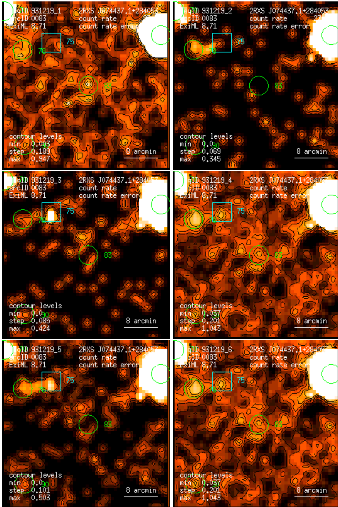
Figure 83: RASS 931219: detection 0083: band rate images, Gaussian filter: (1) PSPC channels 11 – 41, (2) 52 – 90, (3) 91 – 201, (4) 11 – 235, (5) 52 – 201, (6) 11 – 201. Broad band rates in counts/ks. Band rate contour levels in counts/ks/arcmin 2 .
