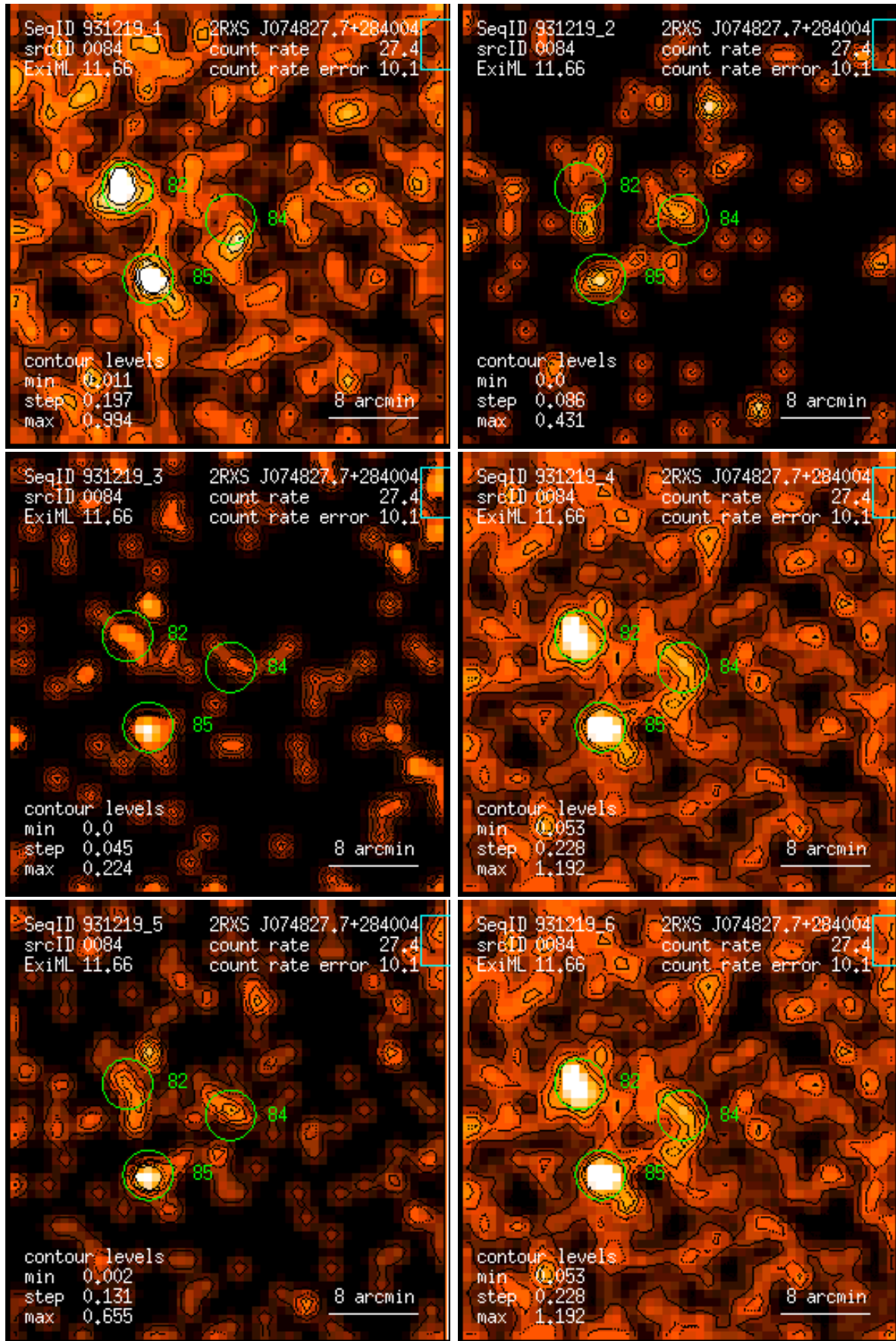
Figure 84: RASS 931219: detection 0084: band rate images, Gaussian filter: (1) PSPC channels 11 – 41, (2) 52 – 90, (3) 91 – 201, (4) 11 – 235, (5) 52 – 201, (6) 11 – 201. Broad band rates in counts/ks. Band rate contour levels in counts/ks/arcmin 2 .
