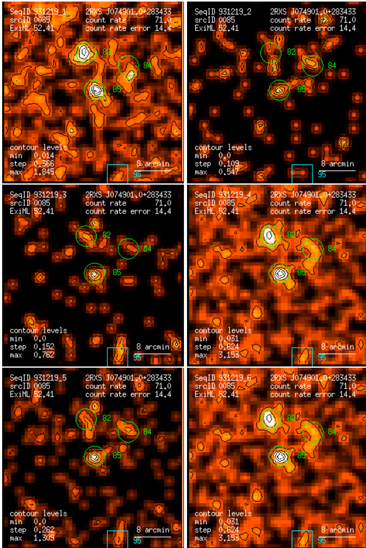
Figure 85: RASS 931219: detection 0085: band rate images, Gaussian filter: (1) PSPC channels 11 – 41, (2) 52 – 90, (3) 91 – 201, (4) 11 – 235, (5) 52 – 201, (6) 11 – 201. Broad band rates in counts/ks. Band rate contour levels in counts/ks/arcmin 2 .
