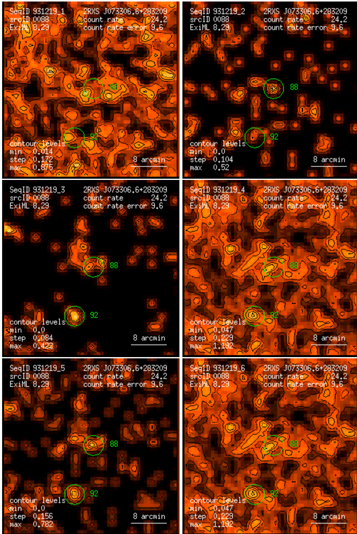
Figure 88: RASS 931219: detection 0088: band rate images, Gaussian filter: (1) PSPC channels 11 – 41, (2) 52 – 90, (3) 91 – 201, (4) 11 – 235, (5) 52 – 201, (6) 11 – 201. Broad band rates in counts/ks. Band rate contour levels in counts/ks/arcmin 2 .
