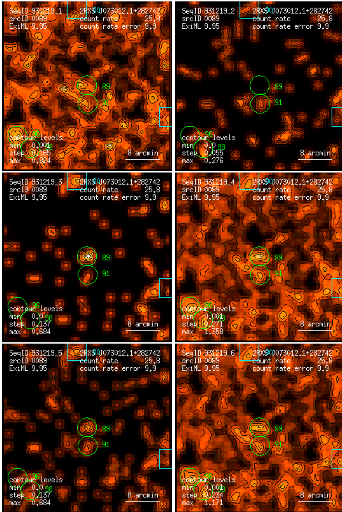
Figure 89: RASS 931219: detection 0089: band rate images, Gaussian filter: (1) PSPC channels 11 – 41, (2) 52 – 90, (3) 91 – 201, (4) 11 – 235, (5) 52 – 201, (6) 11 – 201. Broad band rates in counts/ks. Band rate contour levels in counts/ks/arcmin 2 .
