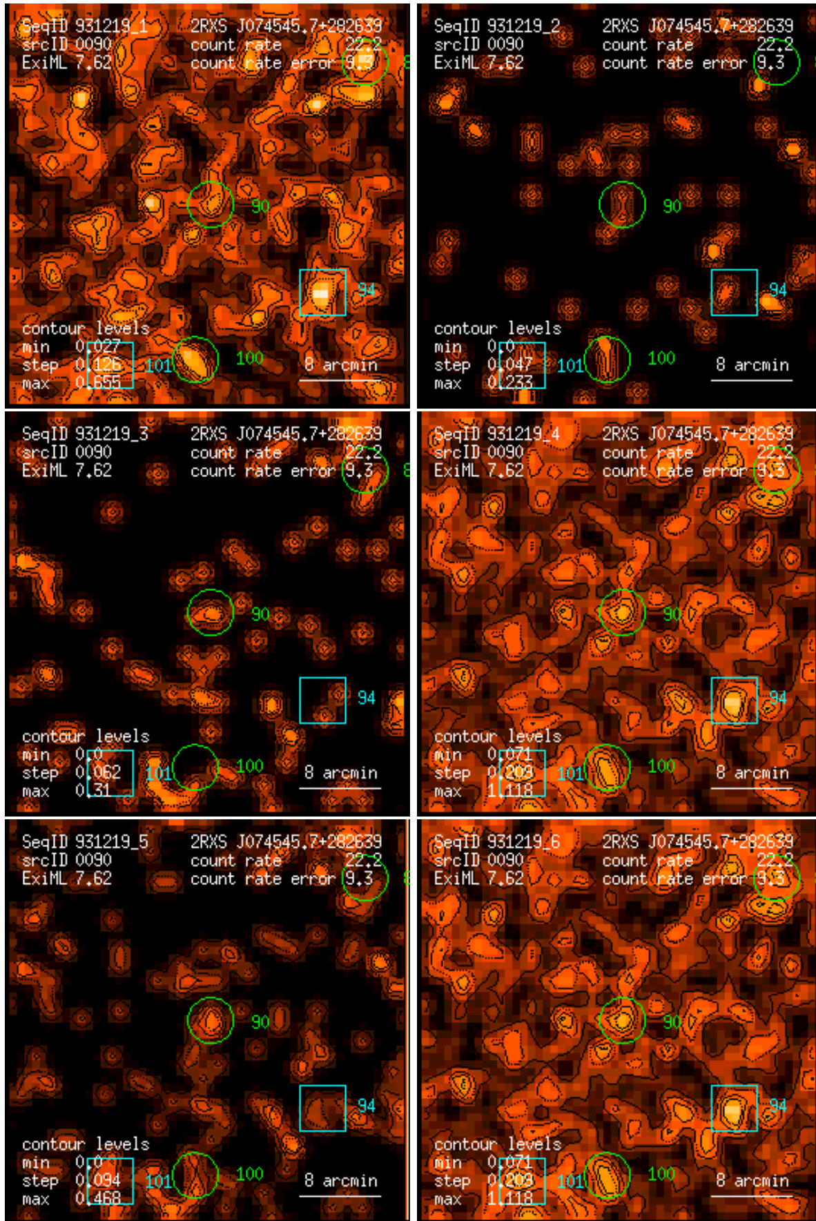
Figure 90: RASS 931219: detection 0090: band rate images, Gaussian filter: (1) PSPC channels 11 – 41, (2) 52 – 90, (3) 91 – 201, (4) 11 – 235, (5) 52 – 201, (6) 11 – 201. Broad band rates in counts/ks. Band rate contour levels in counts/ks/arcmin 2 .
