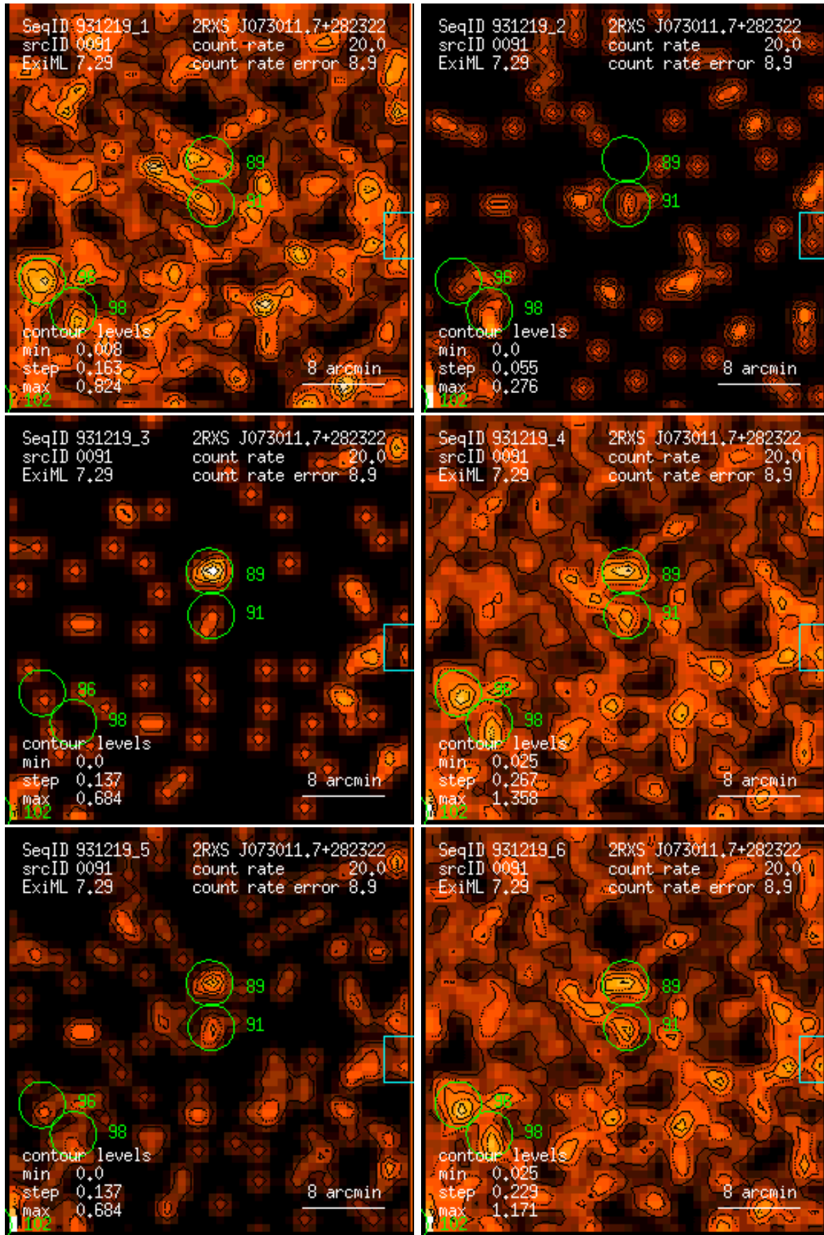
Figure 91: RASS 931219: detection 0091: band rate images, Gaussian filter: (1) PSPC channels 11 – 41, (2) 52 – 90, (3) 91 – 201, (4) 11 – 235, (5) 52 – 201, (6) 11 – 201. Broad band rates in counts/ks. Band rate contour levels in counts/ks/arcmin 2 .
