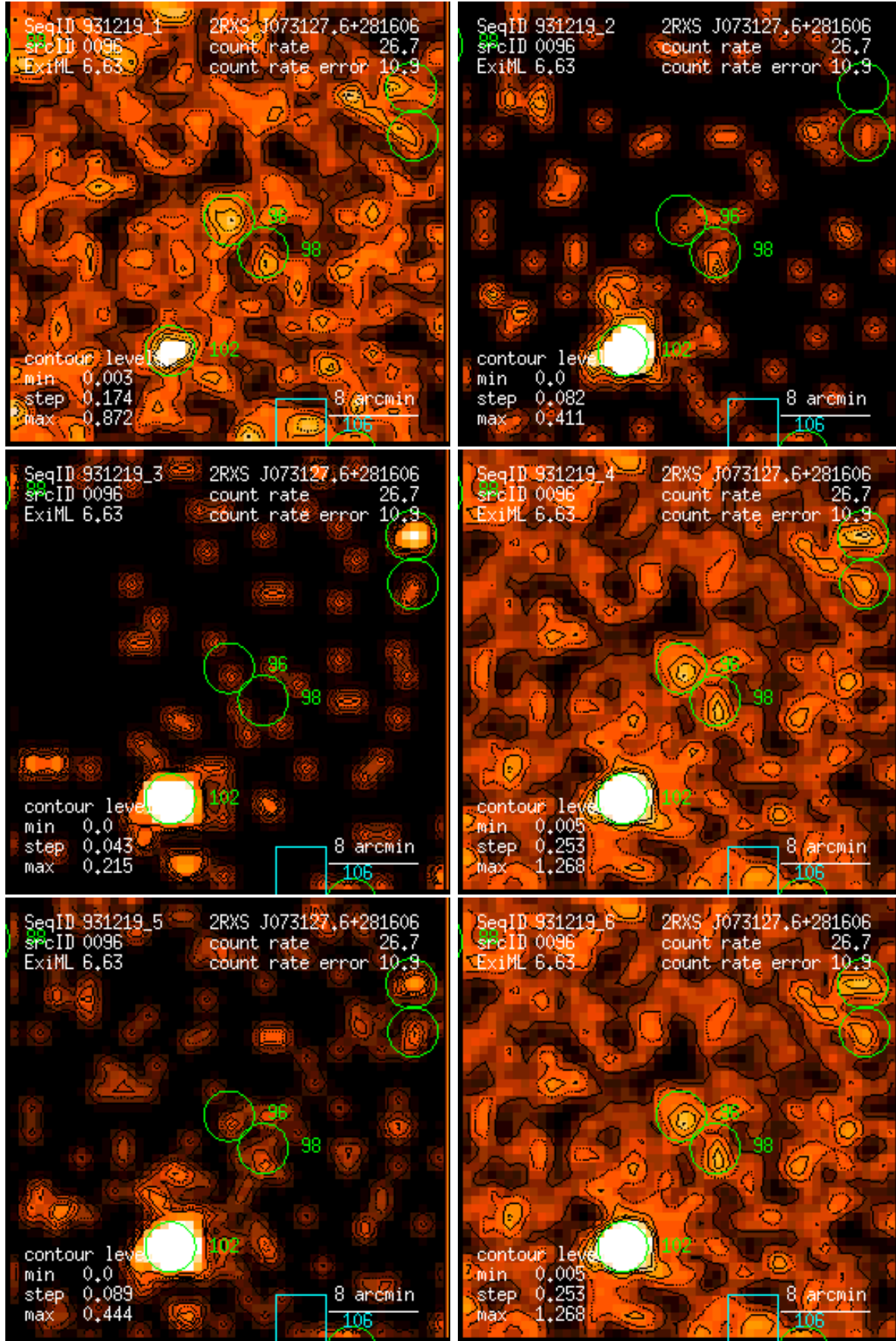
Figure 96: RASS 931219: detection 0096: band rate images, Gaussian filter: (1) PSPC channels 11 – 41, (2) 52 – 90, (3) 91 – 201, (4) 11 – 235, (5) 52 – 201, (6) 11 – 201. Broad band rates in counts/ks. Band rate contour levels in counts/ks/arcmin 2 .
