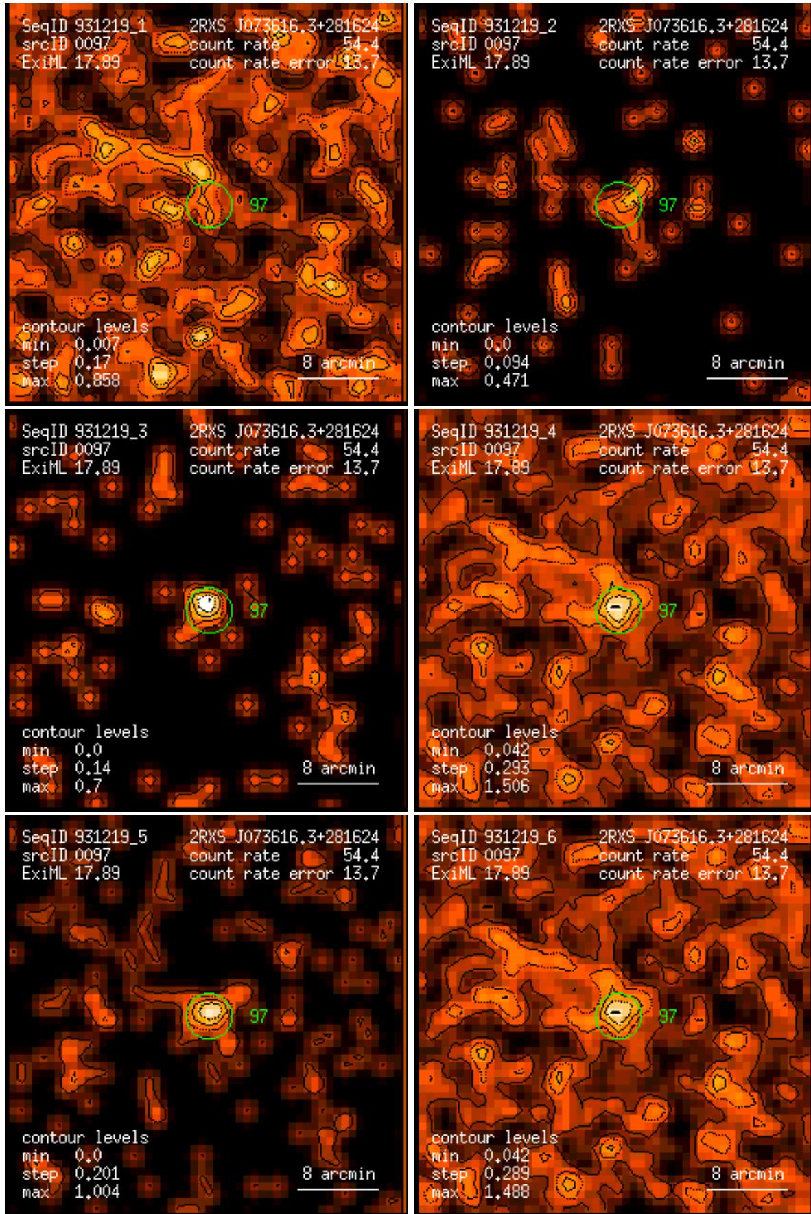
Figure 97: RASS 931219: detection 0097: band rate images, Gaussian filter: (1) PSPC channels 11 – 41, (2) 52 – 90, (3) 91 – 201, (4) 11 – 235, (5) 52 – 201, (6) 11 – 201. Broad band rates in counts/ks. Band rate contour levels in counts/ks/arcmin 2 .
