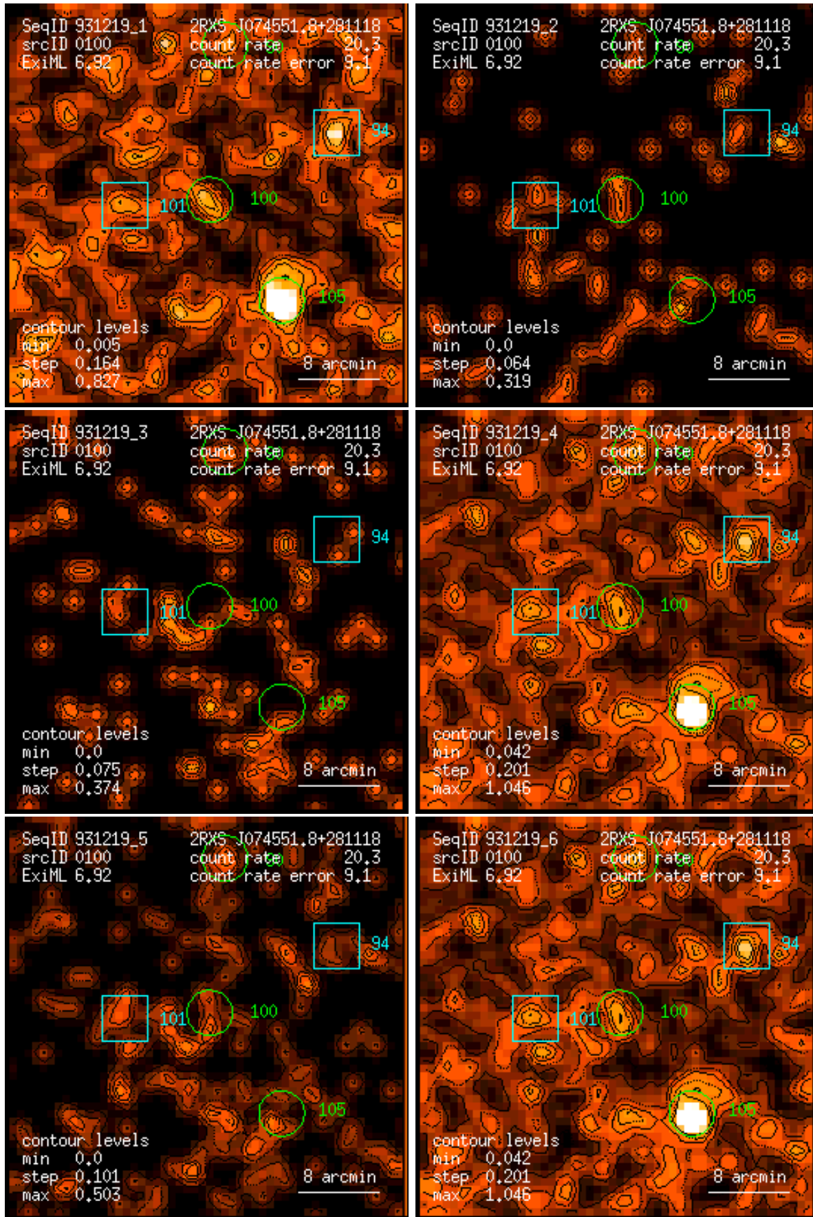
Figure 100: RASS 931219: detection 0100: band rate images, Gaussian filter: (1) PSPC channels 11 – 41, (2) 52 – 90, (3) 91 – 201, (4) 11 – 235, (5) 52 – 201, (6) 11 – 201. Broad band rates in counts/ks. Band rate contour levels in counts/ks/arcmin 2 .
