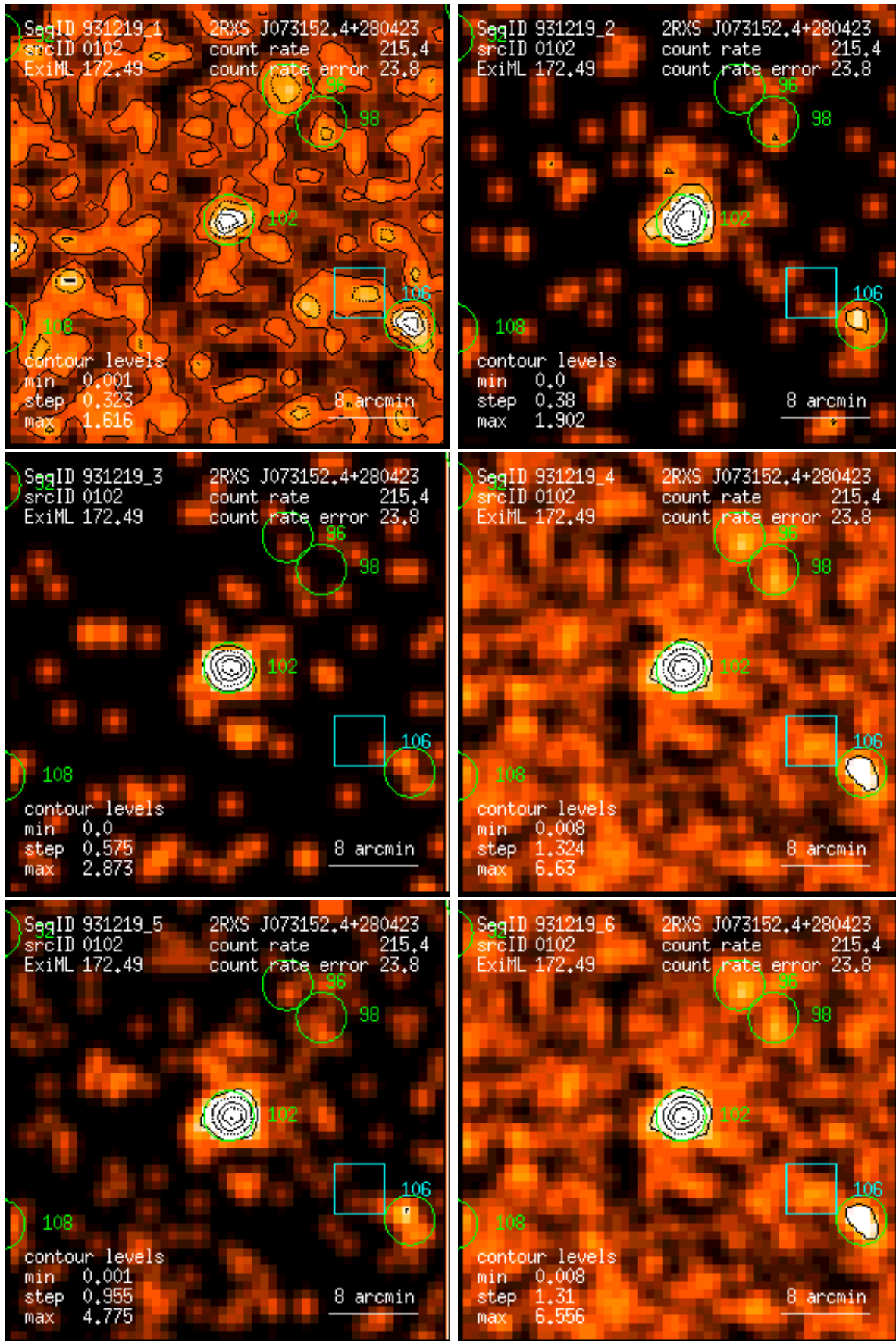
Figure 102: RASS 931219: detection 0102: band rate images, Gaussian filter: (1) PSPC channels 11 – 41, (2) 52 – 90, (3) 91 – 201, (4) 11 – 235, (5) 52 – 201, (6) 11 – 201. Broad band rates in counts/ks. Band rate contour levels in counts/ks/arcmin 2 .
