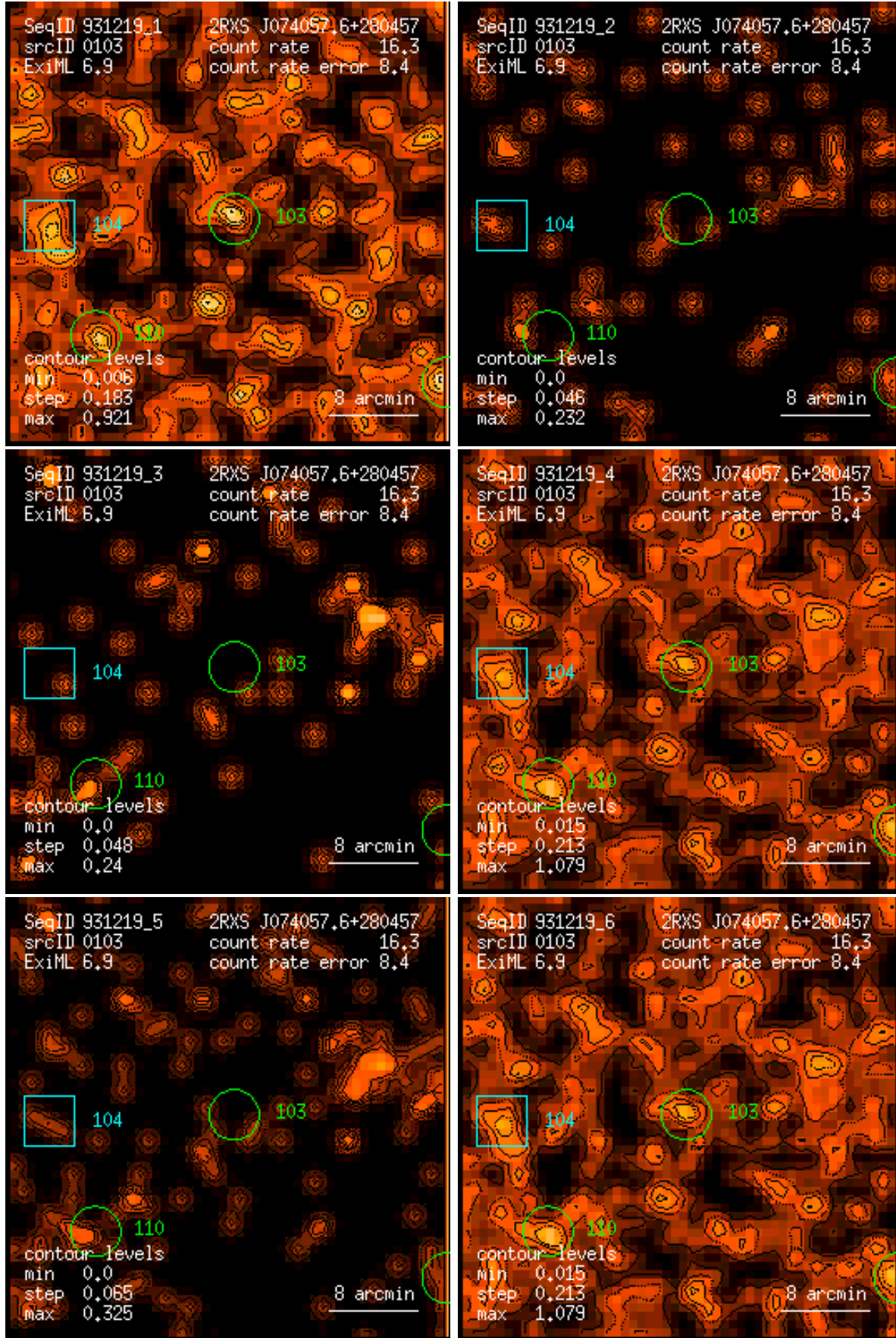
Figure 103: RASS 931219: detection 0103: band rate images, Gaussian filter: (1) PSPC channels 11 – 41, (2) 52 – 90, (3) 91 – 201, (4) 11 – 235, (5) 52 – 201, (6) 11 – 201. Broad band rates in counts/ks. Band rate contour levels in counts/ks/arcmin 2 .
