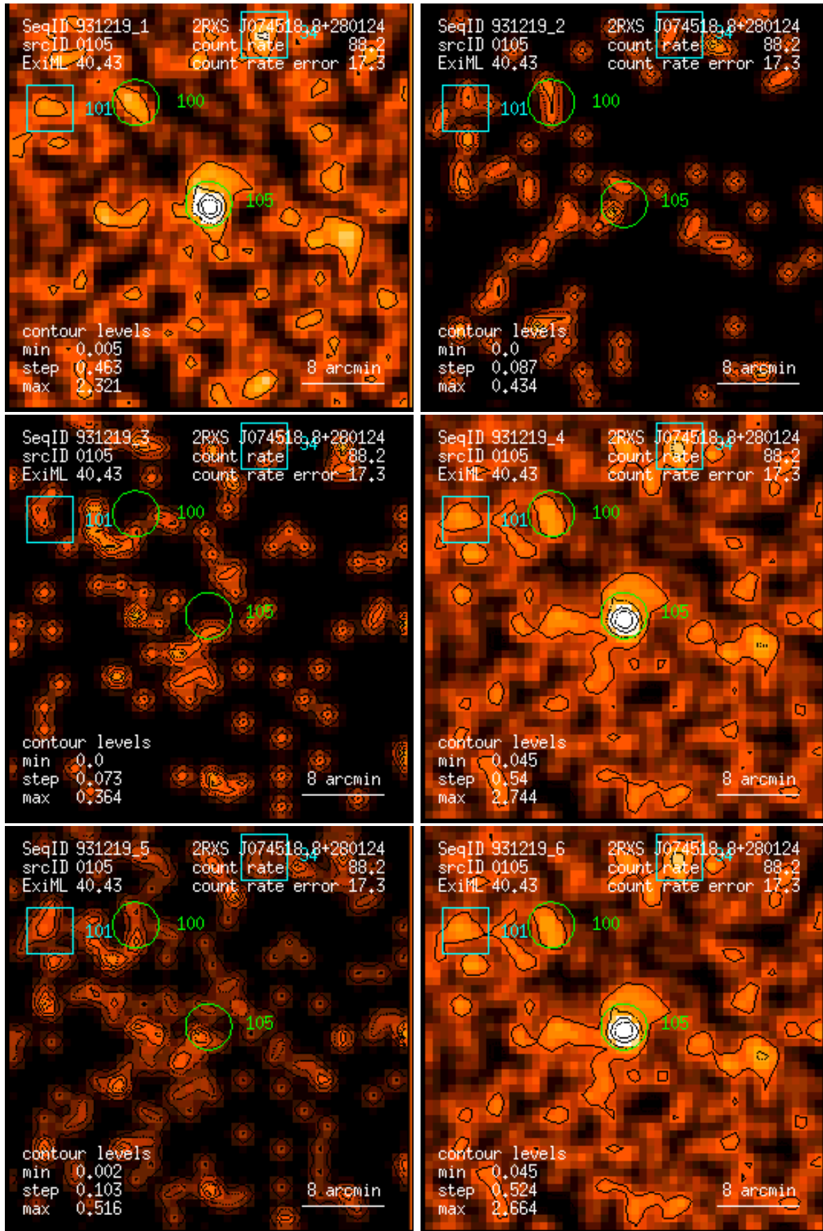
Figure 105: RASS 931219: detection 0105: band rate images, Gaussian filter: (1) PSPC channels 11 – 41, (2) 52 – 90, (3) 91 – 201, (4) 11 – 235, (5) 52 – 201, (6) 11 – 201. Broad band rates in counts/ks. Band rate contour levels in counts/ks/arcmin 2 .
