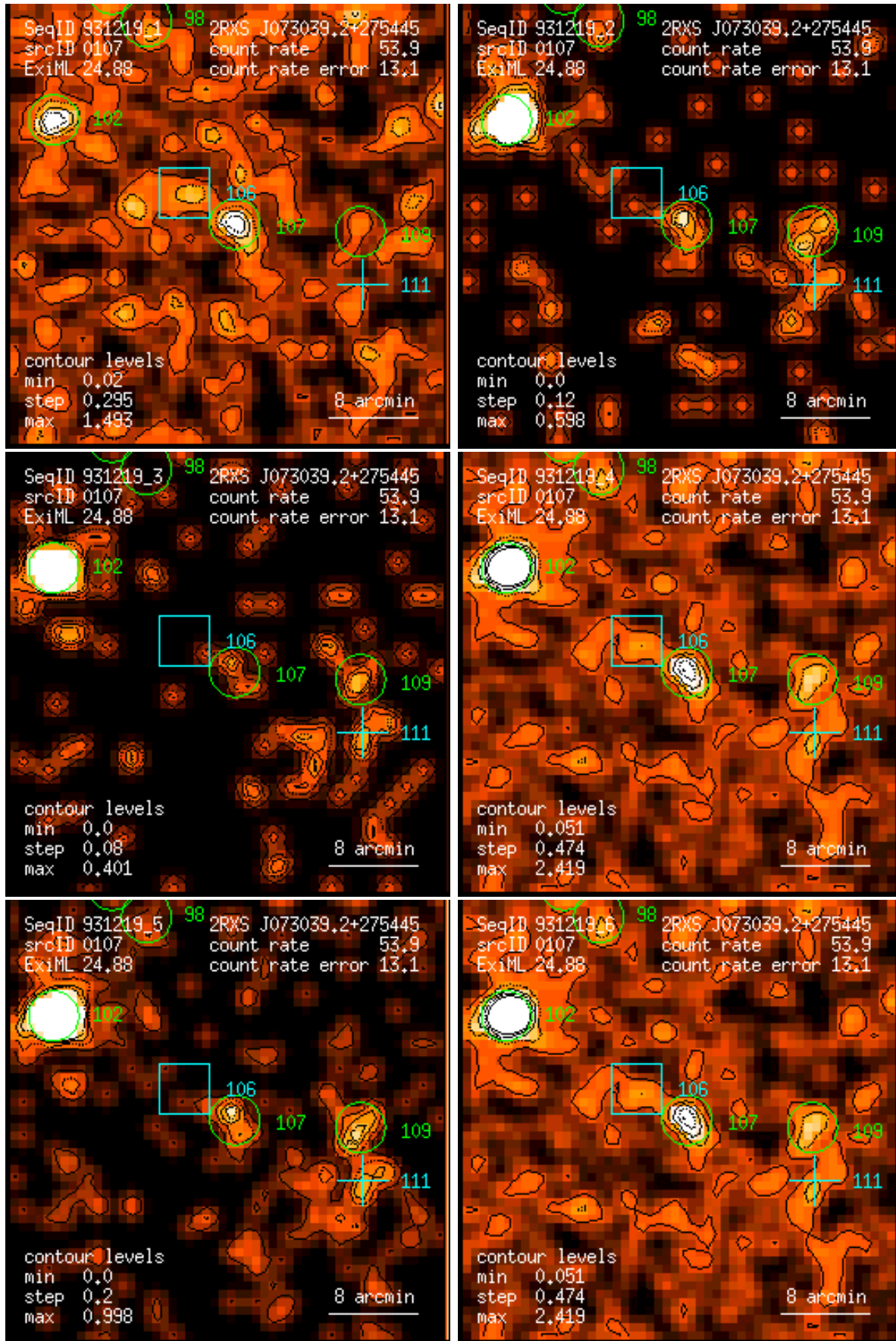
Figure 107: RASS 931219: detection 0107: band rate images, Gaussian filter: (1) PSPC channels 11 – 41, (2) 52 – 90, (3) 91 – 201, (4) 11 – 235, (5) 52 – 201, (6) 11 – 201. Broad band rates in counts/ks. Band rate contour levels in counts/ks/arcmin 2 .
