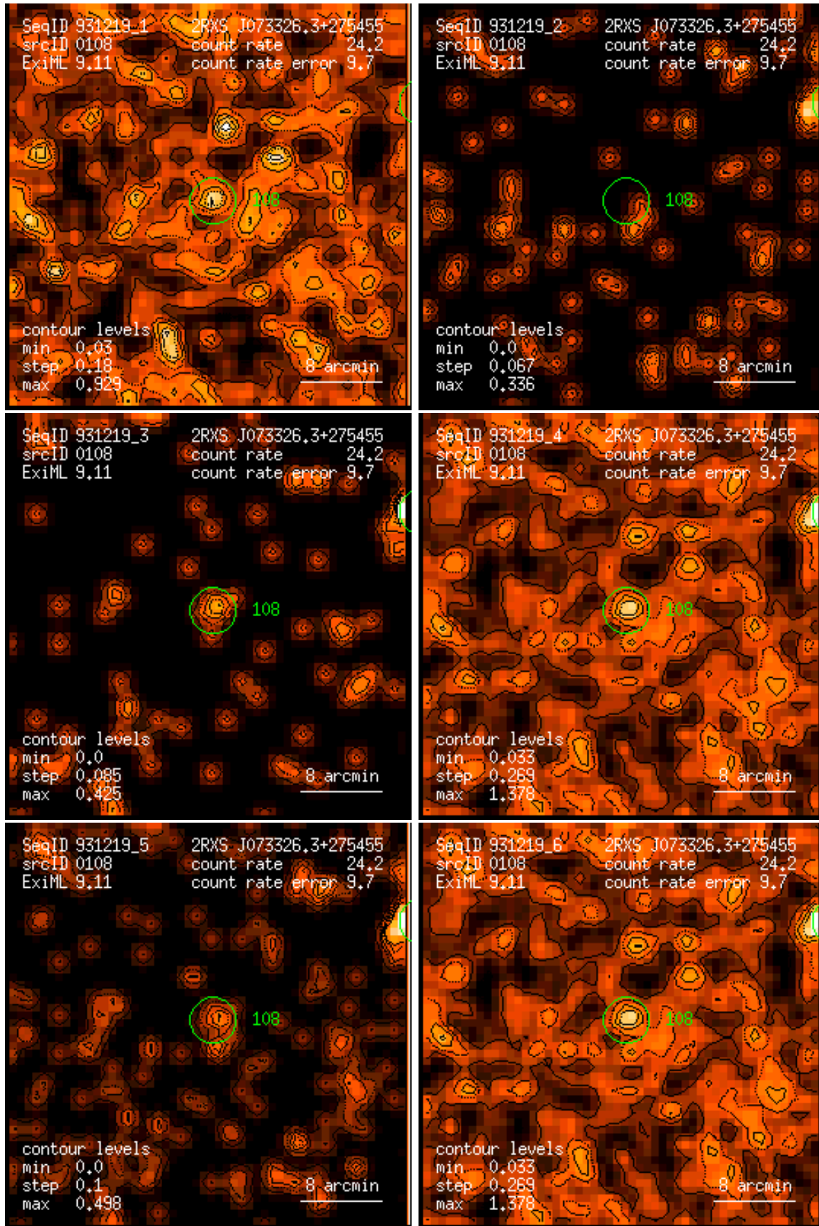
Figure 108: RASS 931219: detection 0108: band rate images, Gaussian filter: (1) PSPC channels 11 – 41, (2) 52 – 90, (3) 91 – 201, (4) 11 – 235, (5) 52 – 201, (6) 11 – 201. Broad band rates in counts/ks. Band rate contour levels in counts/ks/arcmin 2 .
