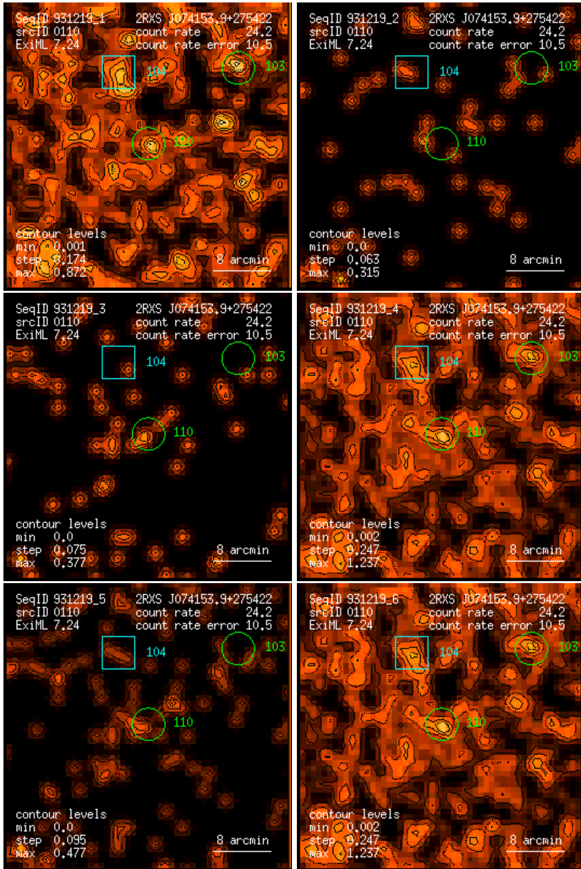
Figure 110: RASS 931219: detection 0110: band rate images, Gaussian filter: (1) PSPC channels 11 – 41, (2) 52 – 90, (3) 91 – 201, (4) 11 – 235, (5) 52 – 201, (6) 11 – 201. Broad band rates in counts/ks. Band rate contour levels in counts/ks/arcmin 2 .
