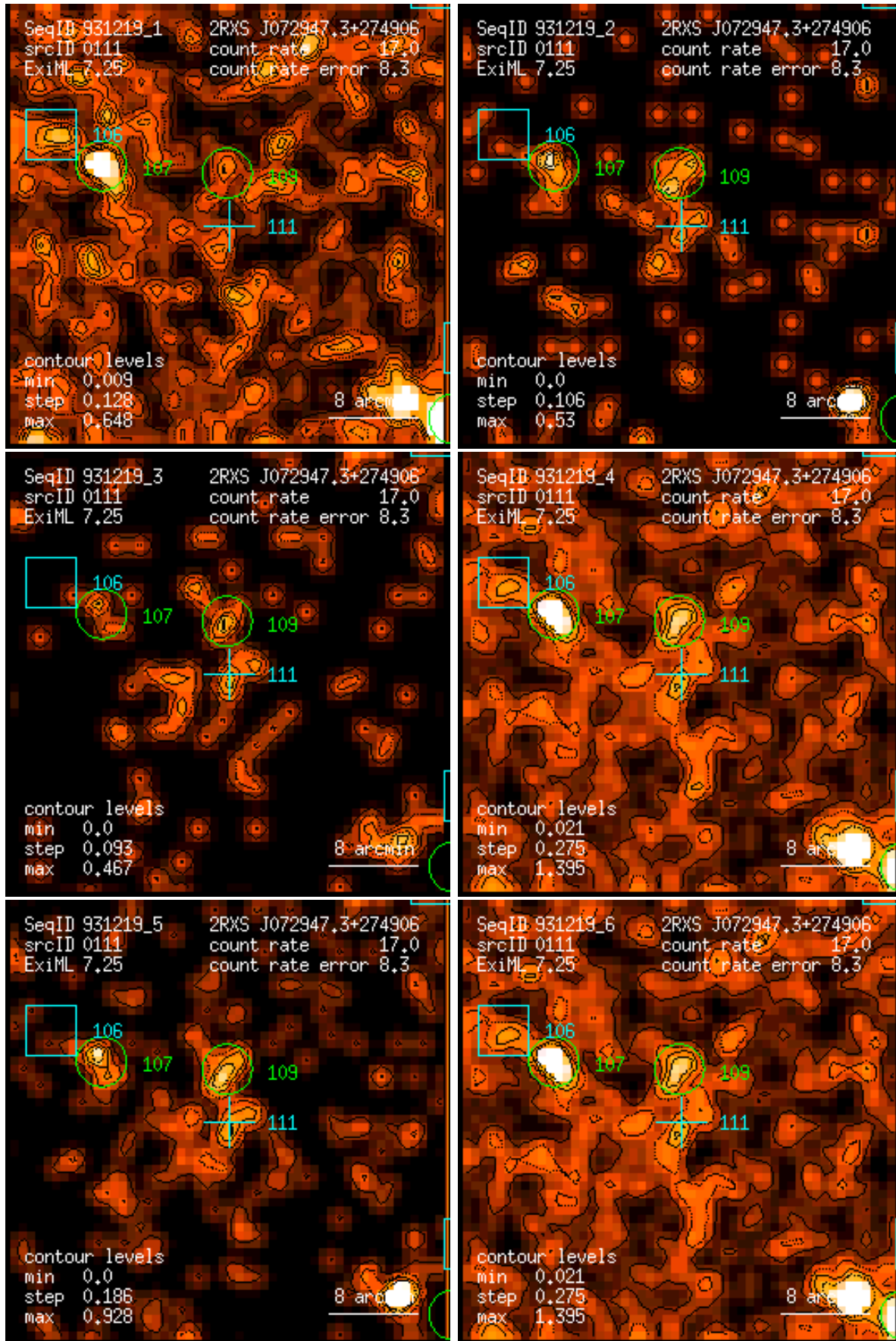
Figure 111: RASS 931219: detection 0111: band rate images, Gaussian filter: (1) PSPC channels 11 – 41, (2) 52 – 90, (3) 91 – 201, (4) 11 – 235, (5) 52 – 201, (6) 11 – 201. Broad band rates in counts/ks. Band rate contour levels in counts/ks/arcmin 2 .
