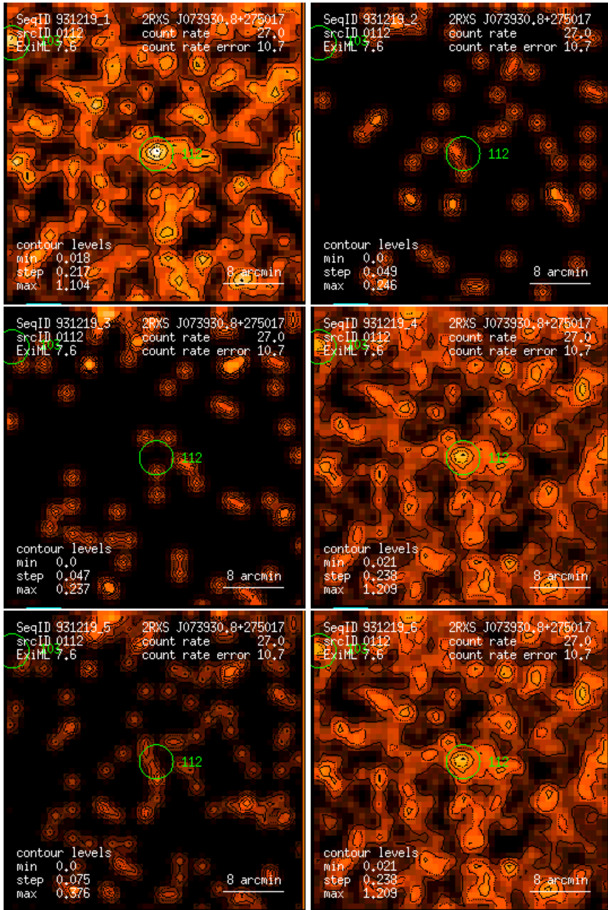
Figure 112: RASS 931219: detection 0112: band rate images, Gaussian filter: (1) PSPC channels 11 – 41, (2) 52 – 90, (3) 91 – 201, (4) 11 – 235, (5) 52 – 201, (6) 11 – 201. Broad band rates in counts/ks. Band rate contour levels in counts/ks/arcmin 2 .
