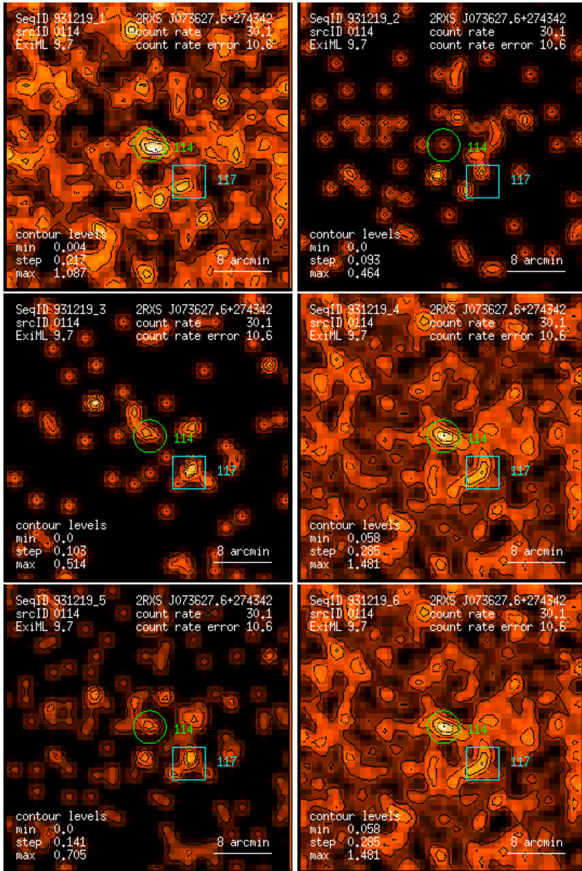
Figure 114: RASS 931219: detection 0114: band rate images, Gaussian filter: (1) PSPC channels 11 – 41, (2) 52 – 90, (3) 91 – 201, (4) 11 – 235, (5) 52 – 201, (6) 11 – 201. Broad band rates in counts/ks. Band rate contour levels in counts/ks/arcmin 2 .
