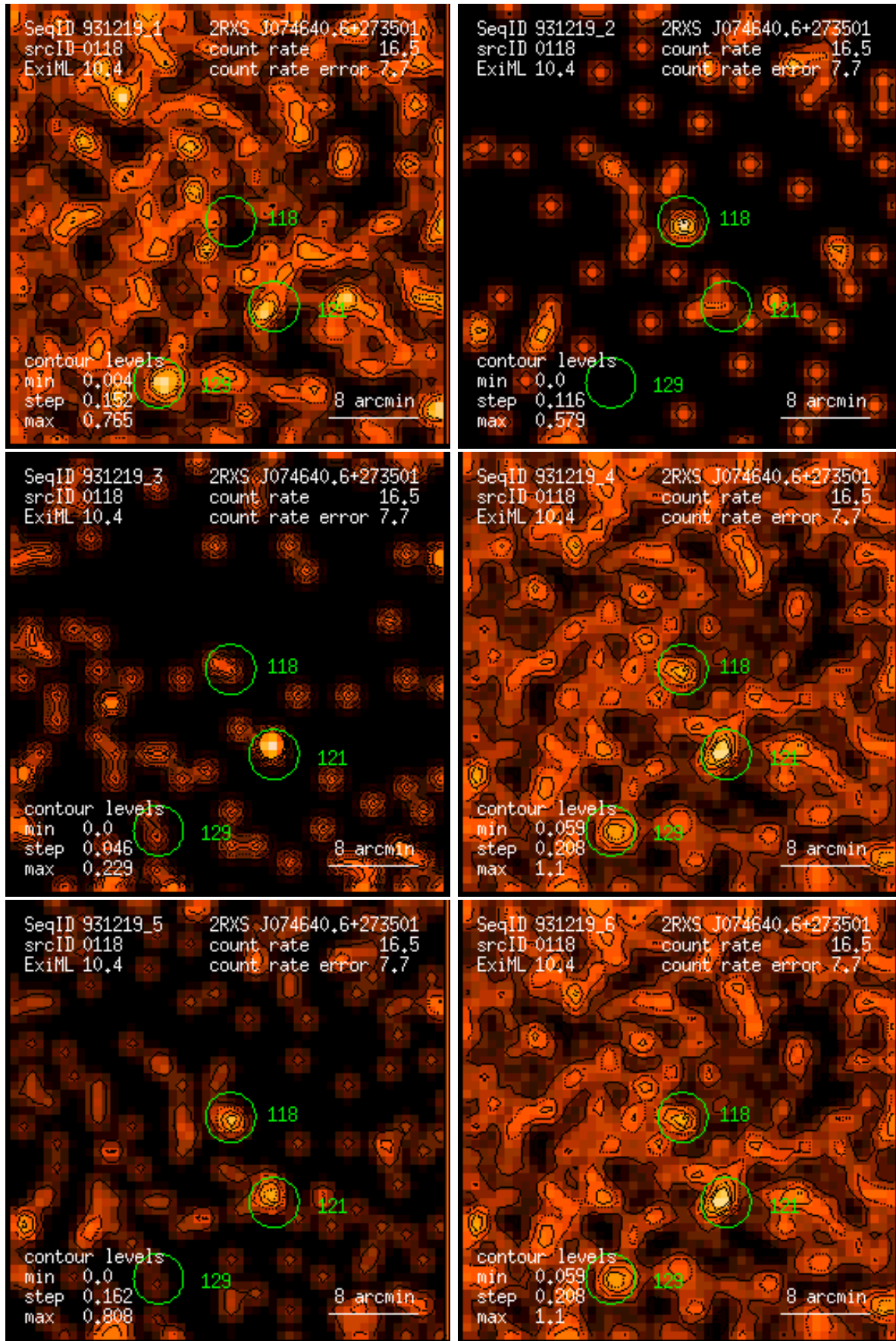
Figure 118: RASS 931219: detection 0118: band rate images, Gaussian filter: (1) PSPC channels 11 – 41, (2) 52 – 90, (3) 91 – 201, (4) 11 – 235, (5) 52 – 201, (6) 11 – 201. Broad band rates in counts/ks. Band rate contour levels in counts/ks/arcmin 2 .
